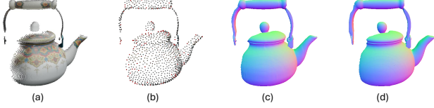
Figure 3. Spatial Locality of 3DShape2VecSet [60] based diffusion models. (a) Given a partial point cloud, (b) we sample query points q using farthest point sampling [34] (c) We encode the point cloud into the latent space with q , and decode it into a mesh. (d) We perform noise inversion [47] and recover the shape through denoising and decoding.
