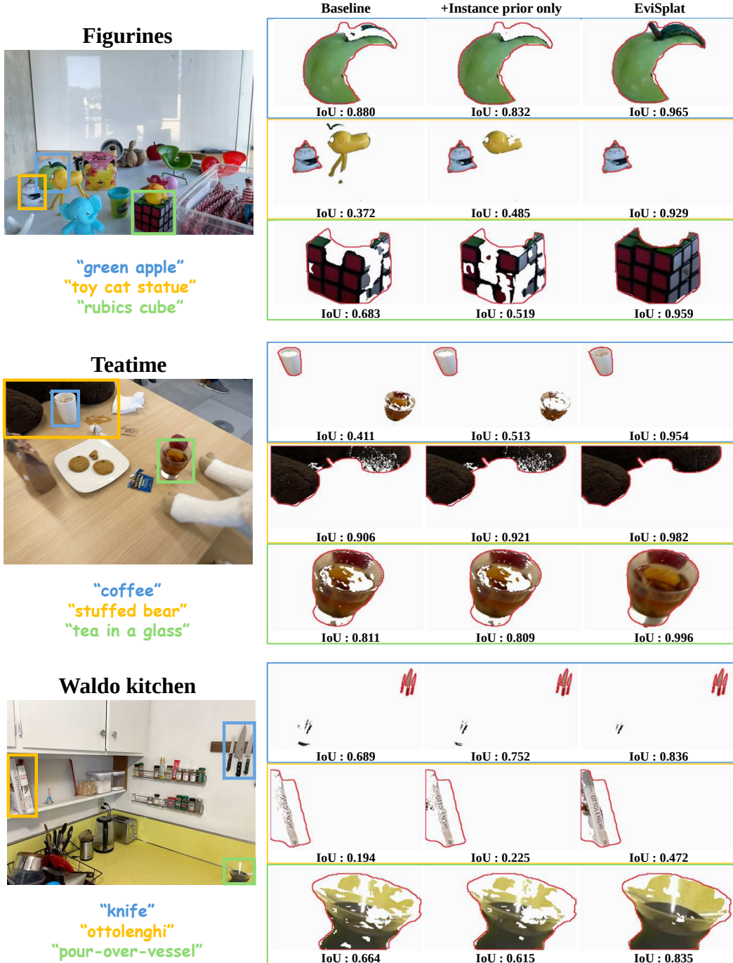
Figure D.1: Qualitative results on LERF-OVS. Baseline, instance prior only, and EviSplat. Red outlines mark ground truth; values report rendered-view mask IoU.
