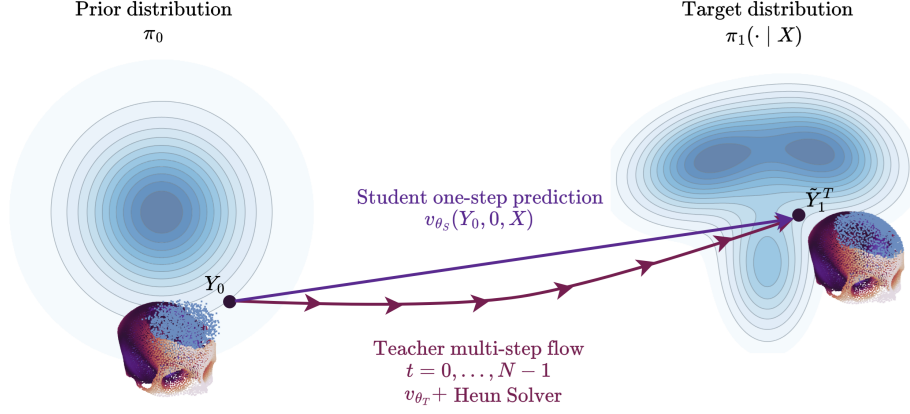
Fig. 1. Teacher-guided Endpoint Distillation (TED). Given defective skull X , the flow is defined only over the implant Y . A prior sample Y_0 \sim \pi_0 is transported by the teacher to endpoint \tilde{Y}_1^T , while the student learns a single-step displacement from Y_0 to the implant prediction conditioned on X . Skull visualizations show conditioning context only.
