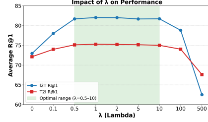
Fig. 3: The impact of lambda. We omit the case without the base loss.
