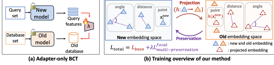
Fig. 1: Overview of MKP-Adapter.
