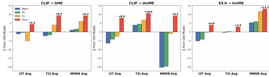
Fig. 2: Histogram of main results. The y-axis shows the performance gap relative to the old model; the black dashed line at zero indicates the old model’s performance. “I2T/T2I AVG” and “MMEB AVG” correspond to the average scores computed over the benchmarks listed in Tab. 1 and Tab. 2, respectively.
