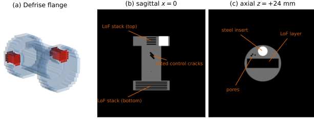
Fig. 2. The Defrise flange phantom. (a) Three-dimensional view of the aluminium body in translucent blue with two press-fit steel inserts in red. (b) Central sagittal slice with the two LoF stacks far off the source plane and the two tilted control cracks in the column. (c) Axial slice through the upper flange disk with the LoF layer, the steel insert, and the pore cluster in the attenuation shadow of the insert.
