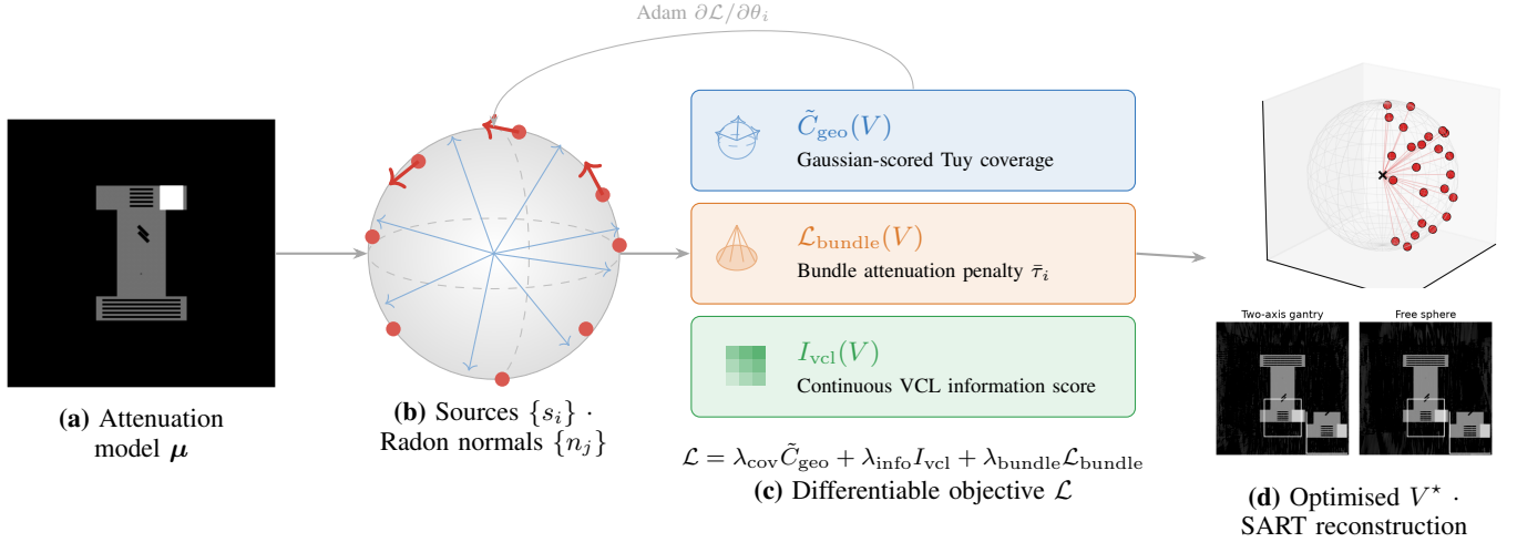
Fig. 1. Overview of the gradient-based trajectory-optimisation pipeline. (a) Attenuation model \mu . (b) The viewing sphere carries two families of symbols. Red dots are the source positions s_i , and blue arrows from the centre are the sampled Radon normals n_j , one for each plane whose coverage is scored. Thick red arrows are the coverage gradient, which is tangential to the sphere by Proposition 2. Every source carries such a gradient, and three are drawn so that the panel stays readable. (c) The objective combines the soft-Tuy coverage surrogate, the attenuation-aware bundle penalty, and the continuous VCL information score; Adam updates the kinematic parameters on the manifold. (d) Two outputs from separate runs. Above, red dots are the optimised source positions V^* of a coverage-only free-sphere run at k=24 , thin red lines are their rays to the region of interest, and the black cross marks its centre. Below, SART reconstructions at k=80 for the two-axis gantry and the free sphere, named in the image.
