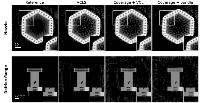
Fig. 5. Noise-free reconstructions at k = 40 , the nozzle rendered at 256 3 for legibility. The top row is a central axial slice of the fuel nozzle with the cooling-hole ring in the inset, the bottom row a central sagittal slice of the Defrise flange with the upper lack-of-fusion stack. The nozzle selections are visually equivalent, as the sub-decibel margins of Table II predict, whereas the flange separates them in the streak background.
