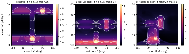
Fig. 3. Directional absorption of the Defrise flange, shown as the bundle path integral \bar{\tau} towards three target points as a function of the source azimuth and elevation on the acquisition sphere. Dark is transparent. Towards the isocentre the transparent region is the equatorial band, since only the column lies in the way there. Towards an off-plane defect the minimum moves into the hemisphere of that defect and leaves a narrow equatorial notch. We aim the term at the isocentre because that choice needs no assumption about which defect matters.
