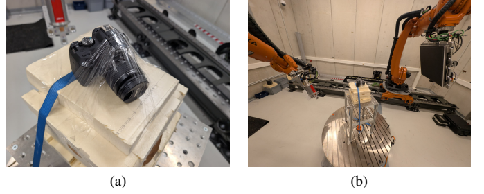
Fig. 4. The scanned object mounted on the rotation stage (a) and the custom robot-based cone-beam CT test bench with the two-axis source and detector manipulators (b).
