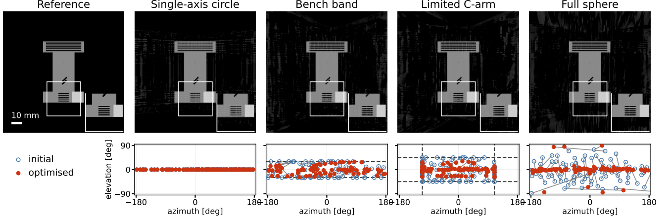
Fig. 6. Defrise flange at k = 80 , native 384^3 . Each geometry column pairs the sagittal reconstruction (top, with LoF inset) with its source poses (bottom). The equatorial circle loses laminar contrast; the bench band already resolves the layers. Open blue circles show Tuy-greedy poses, filled red dots the optimised poses, grey lines their displacement, and dashed lines the reachable limits. Trajectory panels share the elevation scale.
