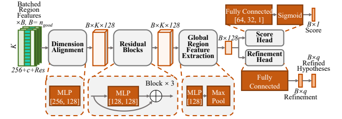
Fig. 6. The architecture of the neural network in the fine-level module. The input data consists of the encoded features of the neighbor region points, forming a batch. Based on the features input to the coarse-level module, the residuals from each point in the neighbor region to its hypothesis are also concatenated. The symbol \oplus denotes element-wise vector addition. The Refinement Head outputs only the increments of the hypothesis parameters, which need to be added to the original hypotheses to obtain the refined hypotheses.
