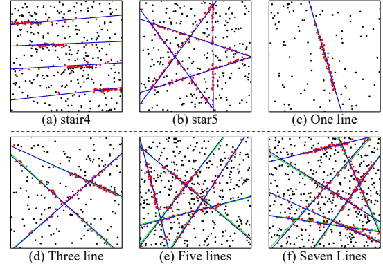
Fig. 9. The qualitative results of LNR on multi-line fitting. The red points represent inliers, while the black points are outliers. The ground truth is represented by green lines, while the fitted lines are represented by blue lines.
