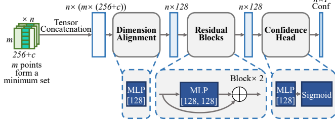
Fig. 4. The architecture of the neural network in coarse-level module. The input data consists of the features of each point in the n minimum sets. The size m of the minimum set varies with the task. The features of each point are concatenated with c -dimensional original features and the extracted 256-dimensional geometric features. The tensor concatenation module concatenates the features of all the points of a minimum set.
