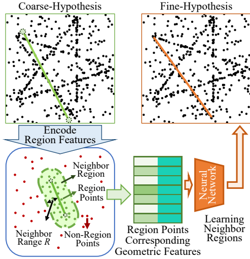
Fig. 5. Encoding region features in fine-level module. Each coarse-hypothesis is encoded region features. The data points within a distance R of the hypothesis are delimited as region points. Geometric features associated with these region points are concatenated as region features, which are learned by the neural network for refinement. Learning the region features of the hypothesis rather than the hypothesis parameters avoids differentiating the sampling process and the model solvers.
