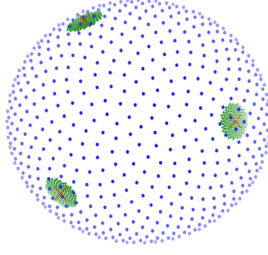
Fig. 7. The similarity between vanishing points. The vanishing points are projected onto a Gaussian sphere and the distances on the sphere are used to compute the similarity between the vanishing points.
