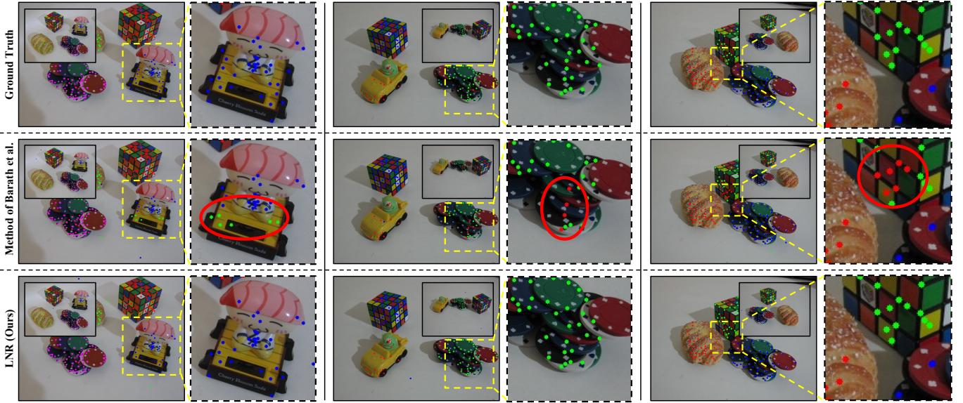
Fig. 13. The qualitative results of the method of Barath et al. [21] and LNR on the two-view motion task in various scenes. Different colors indicate which of the fundamental matrix the correspondences belong to. The small image and the large image are a pair of images. Their correspondences are used as input to the task. The major errors are indicated by red circles.
