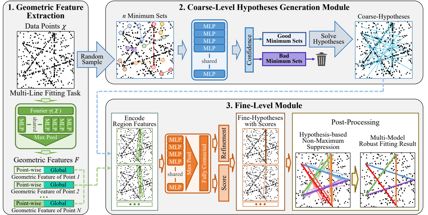
Fig. 2. The pipeline of the proposed LNR. Using the multi-line fitting task as an example. Different colored lines indicate their scores and categories. Two points can form a minimum set to determine a line. LNR consists of three main components: 1. Geometric features are extracted from the data points (Sec. III-A). 2. The quality of randomly sampled minimum sets is evaluated. The good minimum sets are solved into coarse-hypotheses (Sec. III-B). 3. For each coarse-hypotheses, encoding its region feature, which is used for refinement and assessment to get fine-hypotheses (Sec. III-C). Then a Hypothesis-based Non-Maximum Suppression (HNMS) outputs a compound model as the final robust multi-model fitting results (Sec. III-D).
