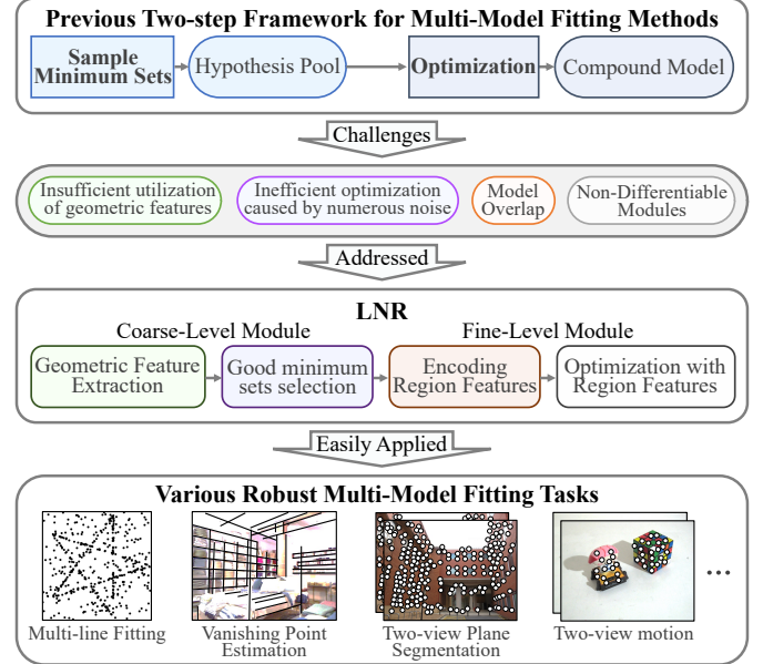
Fig. 1. LNR addresses the challenges of the two-step framework. LNR uses neural network in the coarse module to fully extract geometric features and select good minimum sets for efficiency. In the fine-level module, LNR encodes region features for each hypothesis independently to deal with model overlap. This framework learns on data points rather than the hypothesis parameters, avoiding sampling process and model solvers
