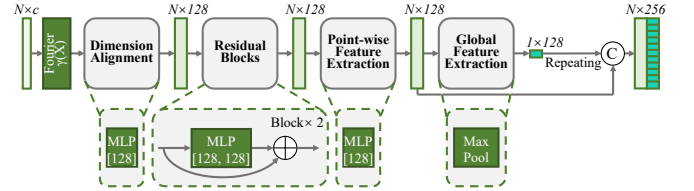
Fig. 3. The architecture of the neural network in geometric feature extraction. Most raw data can be represented as unordered N \times c data points, making the input data N \times c . The symbol \oplus denotes element-wise vector addition, while “C” denotes vector concatenation. The network output is 256-dimensional, comprising 128-dimensional point-wise features concatenated with 128-dimensional global features.
