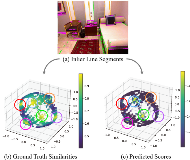
Fig. 12. Score visualization for the vanishing point estimation task. (a) Line segments belonging to different vanishing points are indicated by different colors. All hypothetical vanishing points are projected on a Gaussian sphere (b) and (c). In (b), the linear similarities of the hypotheses to the ground truth are indicated by different colors. In (c), the scores for the hypotheses evaluated by LNR are also indicated by different colors. The same vanishing points in (b) and (c) are marked by the same color circles. LNR assigns high scores to correct hypotheses while greatly suppressing the scores of incorrect hypotheses, better than the linear similarities.
