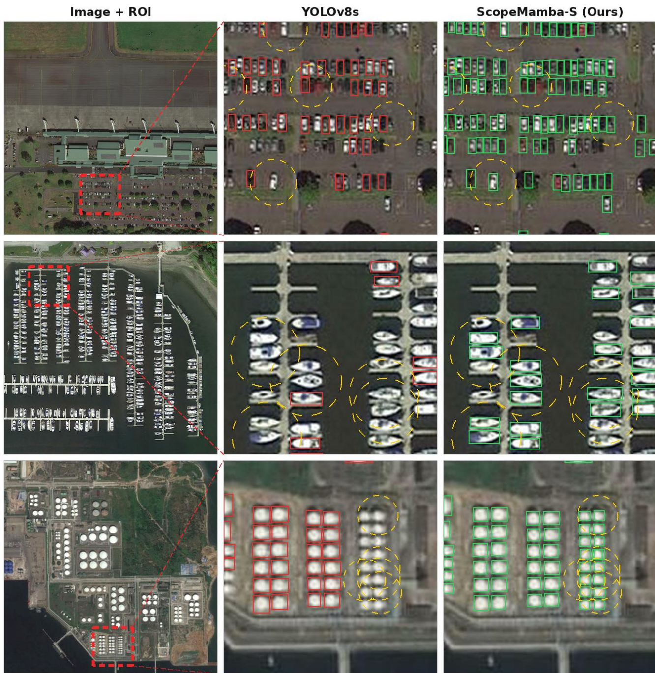
Fig. 8. Qualitative detection results on the AI-TOD validation set. Yellow dashed circles indicate representative ground-truth targets missed by YOLOv8s but detected by ScopeMamba-S in dense or very-tiny object regions.
