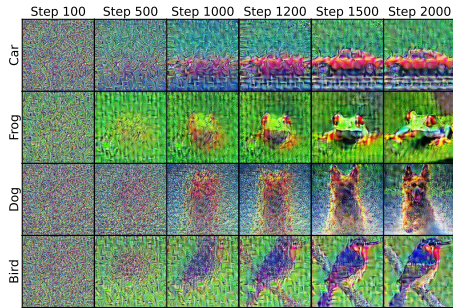
Fig. 1: Small latent diffusion model. SDS with a low-resolution latent diffusion model still produces structured artifacts, suggesting that tensor shape alone does not explain the failure mode.
