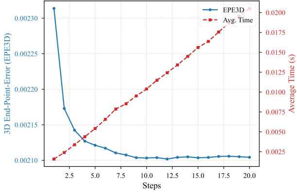
Fig. 3. The effect of inference steps on EPE3D and average inference time
