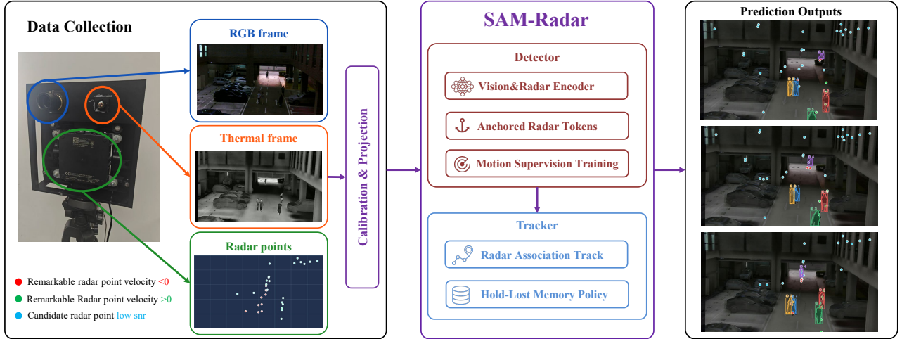
Figure 1: Overview of the acquisition and SAM-Radar pipeline. A rigid rig records calibrated RGB, thermal, and radar streams. The detector fuses visual features with spatially anchored radar tokens trained by motion supervision, and the tracker combines radar association with Hold-Lost memory to produce temporally consistent masks and identities.
