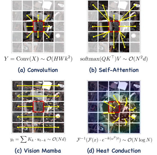
Fig. 1. Comparison of mainstream modeling mechanisms. (a) Convolution. (b) Self-Attention. (c) Vision Mamba. (d) Heat Conduction.
