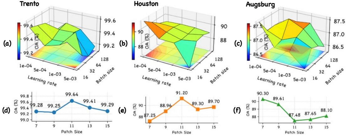
Fig. 4. Impact of hyperparameter selection on the model. (a)–(c) OA variations under different learning rates and batch sizes on the Trento, Houston2013, and Augsburg datasets, respectively; (d)–(f) OA variations under different patch sizes.
