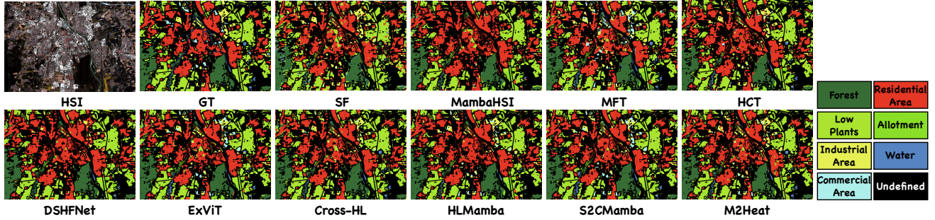
Fig. 7. Classification result mapping by different models on the Augsburg dataset.
