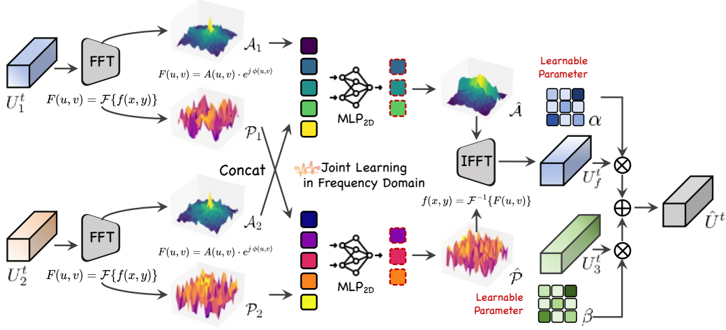
Fig. 3. Our proposed CFF module, which integrates fusion in the frequency domain and dynamic fusion with jointly learned features, enabling effective multimodal feature interaction and fusion.
