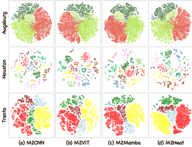
Fig. 8. t-SNE visualization on Trento, Houston, and Augsburg datasets. (a) M2CNN: HCO replaced by a convolution. (b) M2ViT: HCO replaced by MSA. (c) M2Mamba: HCO replaced by Mamba. (d) M2Heat: the proposed method.
