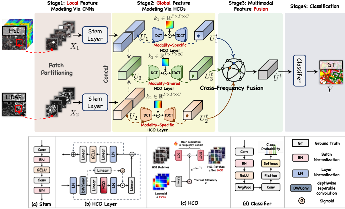
Fig. 2. Overall framework of the proposed M2Heat, which consists of Stem Layer, Modality-specific and Modality-shared HCO Layer, CFF module, and classifier.
