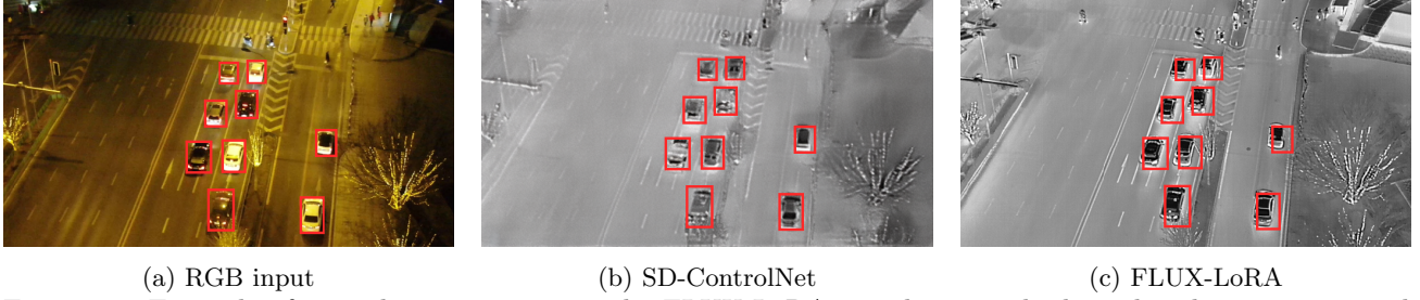
Figure 11: Example of spatial inconsistency in the FLUX-LoRA translation. The bounding boxes correspond to the original RGB annotations. SD-ControlNet preserves the vehicle locations, while FLUX-LoRA shifts the vehicles, causing the transferred annotations to become misaligned.
