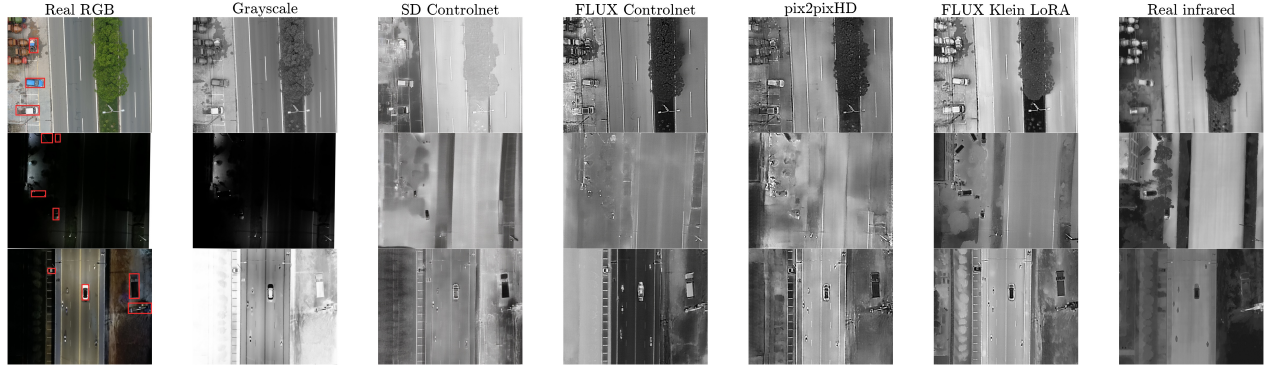
Figure 7: Three RGB-to-IR translation example scenes of the Kust4K training set. From left to right, each row shows an RGB image, the translations generated by the grayscale baseline, SD-ControlNet, FLUX-ControlNet, pix2pixHD, and FLUX-LoRA, and the corresponding real infrared images.
