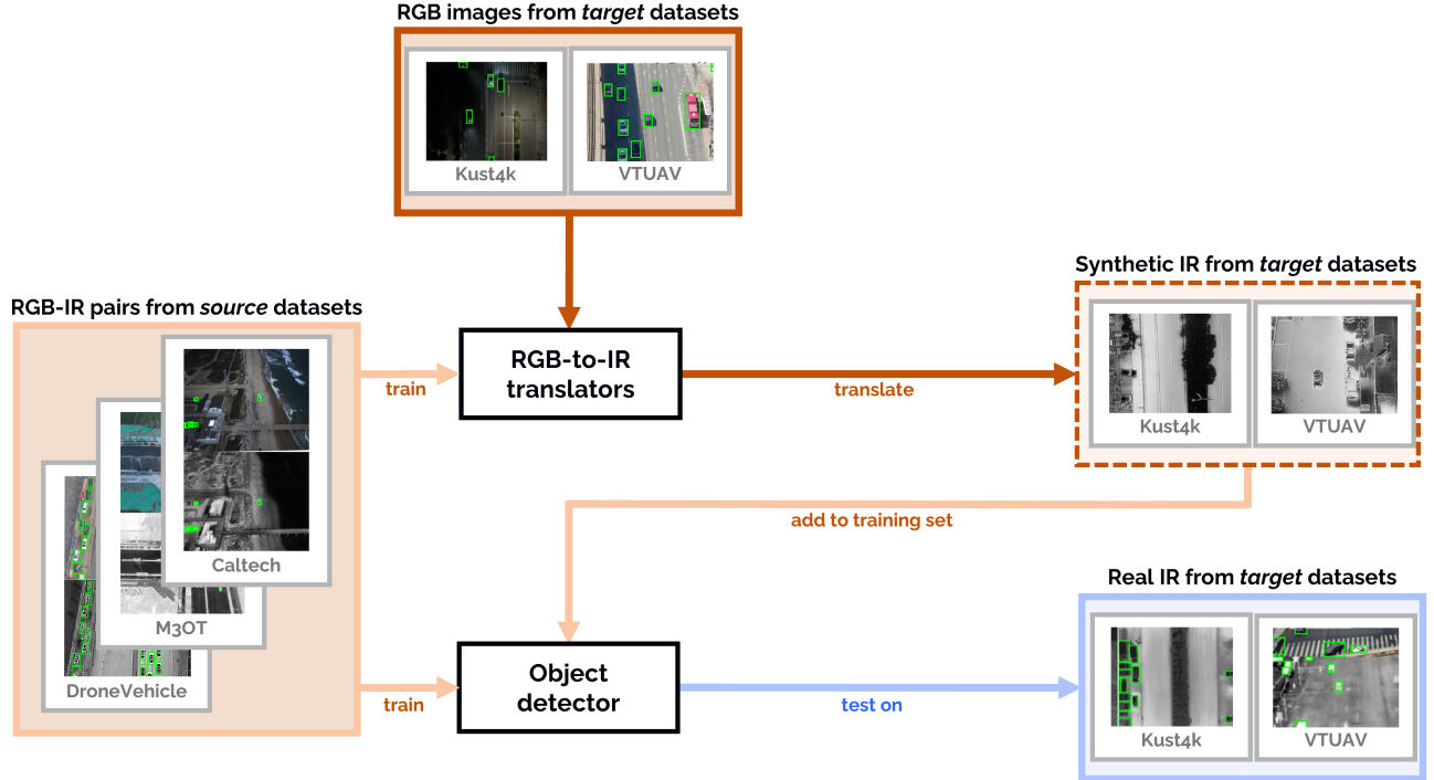
Figure 1: Overview of the proposed workflow. Paired RGB–infrared source datasets (DroneVehicle, Caltech, and M3OT) are used to train RGB-to-IR translation models. These models are subsequently applied to RGB imagery from the training splits of target datasets unseen during translation-model training (Kust4K and VTUAV) to generate synthetic infrared training data. The generated infrared imagery is added to the detector training set, and detection performance is evaluated on real infrared imagery from the separate target-domain evaluation splits. Orange indicates training data and blue indicates evaluation data.
