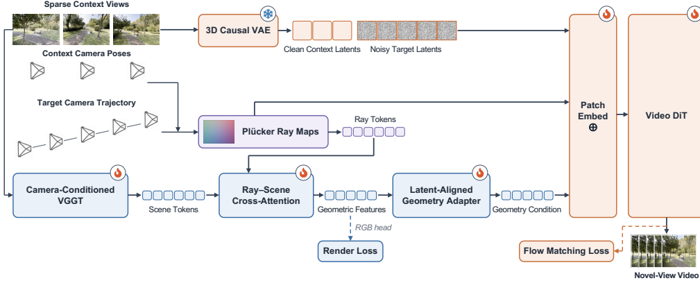
Figure 1: Overview of RoGe. Given sparse posed images and a target camera trajectory, the camera-conditioned VGGT builds an implicit scene representation. Target rays query this representation to extract geometric cues, which are injected into the video diffusion model to synthesize a photorealistic novel-view video. The reconstruction and generation models are trained end-to-end.
