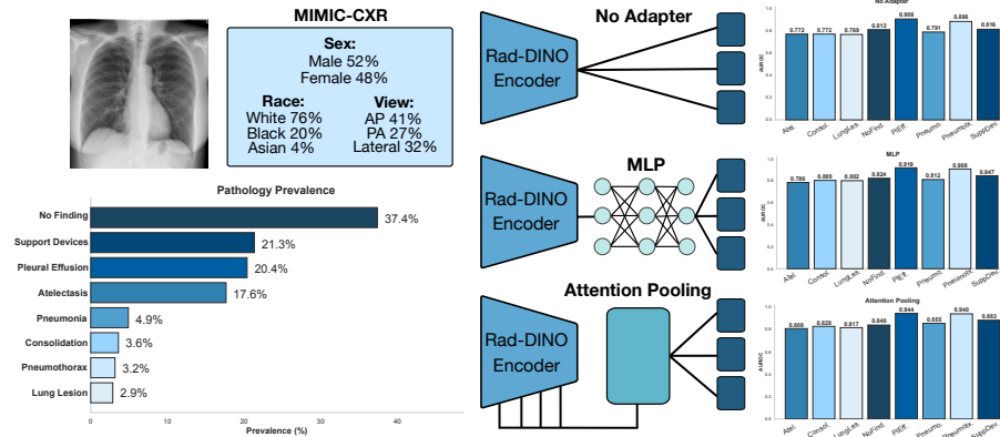
Fig. 1. Overview of the dataset and adapter architectures used to evaluate demographic and imaging-view bias on top of the frozen Rad-DINO foundation model backbone. Three adapter variants are considered, all paired with linear decision heads for downstream pathology classification: 1) No Adapter , using the 768-dimensional CLS token from the final encoder layer directly; 2) an MLP applied to the same CLS token; and 3) an Attention Pooling adapter over features concatenated from four transformer layers across the encoder. Overall AUROC per pathology is reported on the resampled test set used throughout this work.
