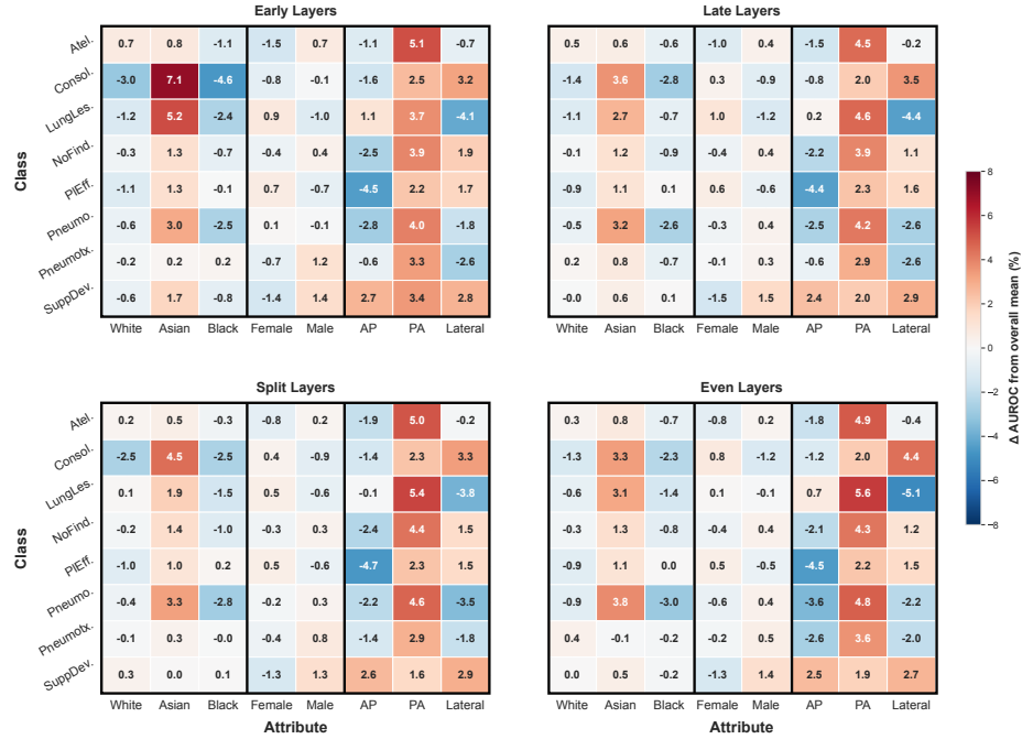
Fig. 3. Subgroup performance characteristics across four different layer combinations used for the attention pooling adapter on the Rad-DINO backbone. Values are reported as percentage AUROC differences from the mean across each pathology.
