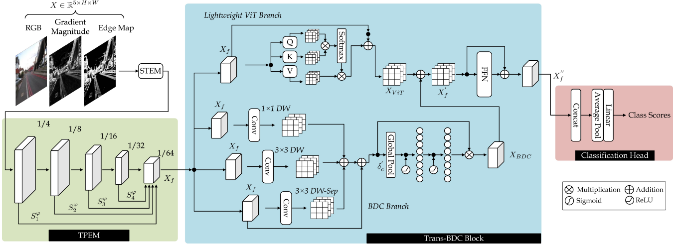
Fig. 4. The architecture of the proposed SiConMo model for the task of image classification.
