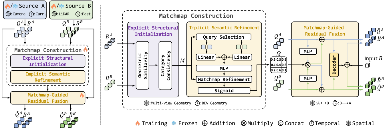
Fig. 2: Architecture of MatchFusion for spatio-temporal interaction through unified instance matching and fusion.
