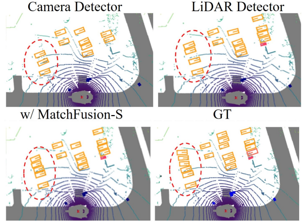
Fig. 3: Qualitative BEV detection results of MatchFusion-S on the nuScenes validation set. Results are shown for the camera front-end Sparse4Dv3, the LiDAR front-end TransFusion-L, and the MatchFusion-equipped system.
