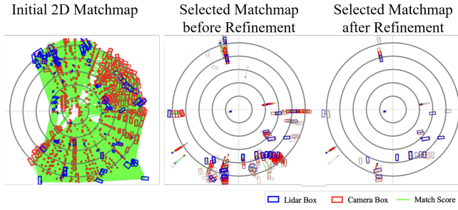
Fig. 4: Qualitative visualization of explicit-implicit cross-modal matching on the nuScenes validation set. Box thickness represents detection confidence, and line thickness represents matching score.
