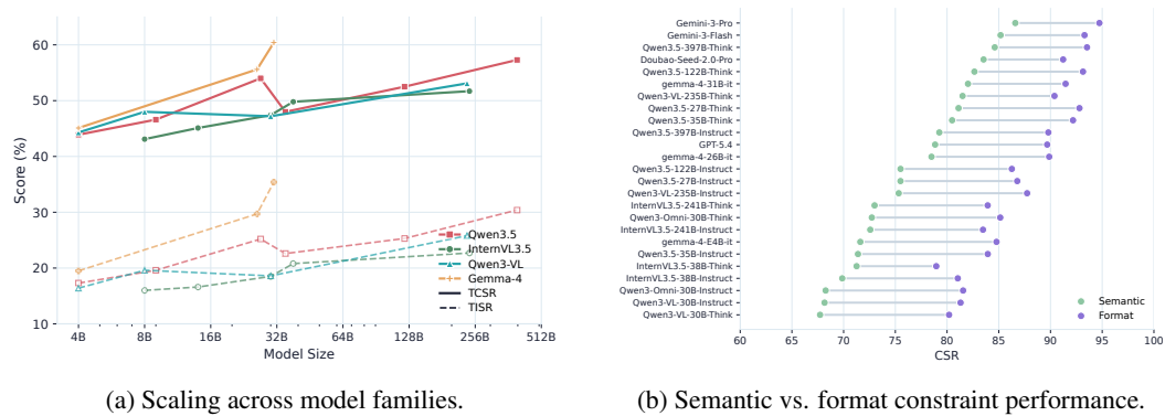
Figure 5: Model scaling and semantic-format constraint performance.
