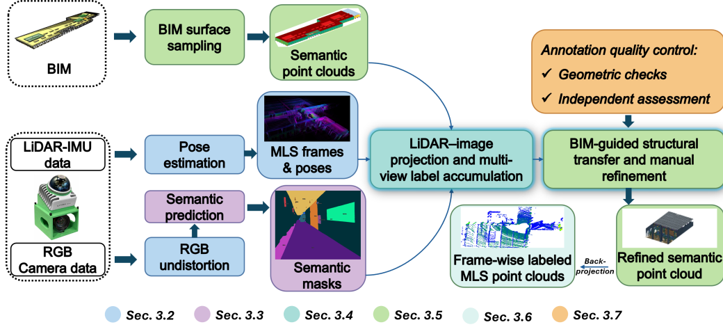
Figure 1: Overview of the dataset construction and annotation workflow, from BIM, LiDAR-IMU data, and camera data to a global semantic point cloud and frame-wise semantic point clouds.
