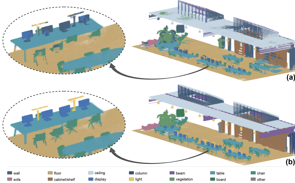
Figure 3: Semantic point cloud example before and after manual refinement, with enlarged local regions. The enlarged regions highlight label corrections around display, chair, and light classes. The before result is obtained after multi-view label accumulation and BIM-guided transfer. (a) Before manual refinement. (b) After manual refinement.
