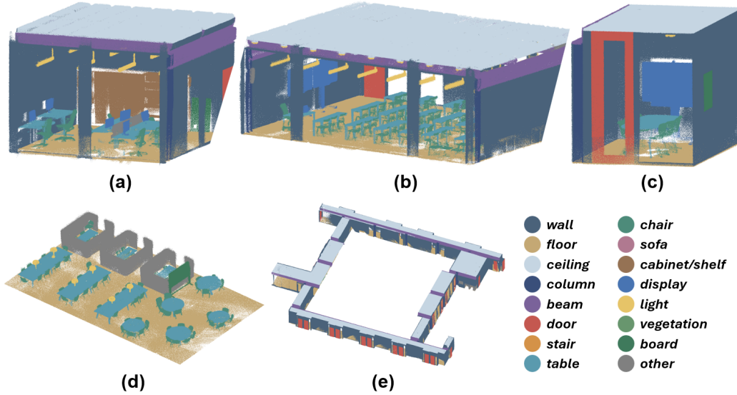
Figure 4: Representative final semantic point clouds from different indoor scene types. (a) Office. (b) Classroom. (c) Meeting room. (d) Study area. (e) Corridor. Panels (d) and (e) are cropped to show the scene structure more clearly.
