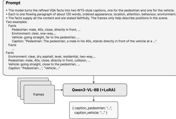
Fig. 3: Structure of the caption generation prompt. The refined VQA facts and the sampled frames are both fed to Qwen3-VL-8B, which returns the pedestrian and vehicle captions as a single JSON object.
