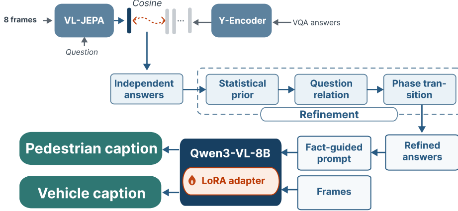
Fig. 2: Refinement and caption generation. The independent VQA answers pass through the training-free refinement (statistical prior, question relation, and phase transition), and the refined answers become facts that, together with the frames, guide Qwen3-VL-8B to write the pedestrian and vehicle captions.
