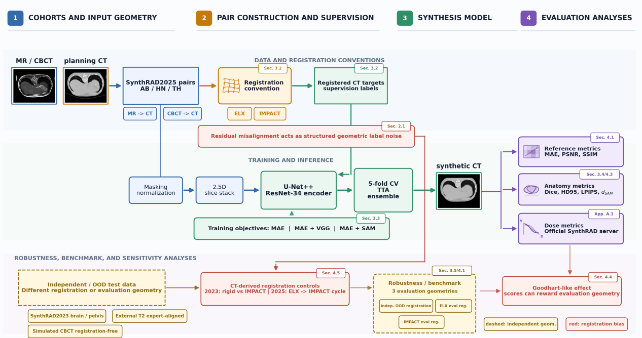
Fig. 1. Overview of the synthesis and evaluation protocol used to study registration-induced bias. Paired MR/CBCT and planning CT data are first converted into supervised training pairs through ELX or IMPACT registration conventions, yielding registered CT targets used as supervision labels for a 2.5D U-Net++ trained with MAE, VGG, or SAM-based objectives. Rectangular blocks denote data, targets, or outputs, whereas rounded blocks denote processing modules, training components, metrics, or analysis toolboxes; dashed blocks indicate independent or OOD evaluation geometries. The resulting synthetic CT images are evaluated using reference-based, anatomy-oriented, and dose-based metrics, complemented by independent/ODD test settings and CT-derived controls that isolate robustness and registration-induced metric sensitivity. Small tags indicate where the corresponding protocol components and analyses are defined in the manuscript. The robustness and benchmark branch distinguishes the independent/ODD geometry from ELX- and IMPACT-based evaluation registrations.
