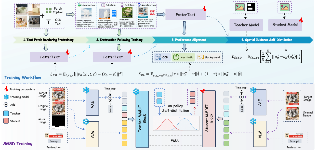
Figure 2: Overview of PosterText. PosterText is trained through four stages: text patch rendering pretraining, instruction-following training, reinforcement learning with human preferences, and Spatial Guidance Self-Distillation (SGSD). The framework supports four operations: generation, addition, deletion, and modification. For SGSD training, the teacher model uses mask-guided inputs for spatial supervision, while the student learns mask-free localization through on-policy self-distillation.
