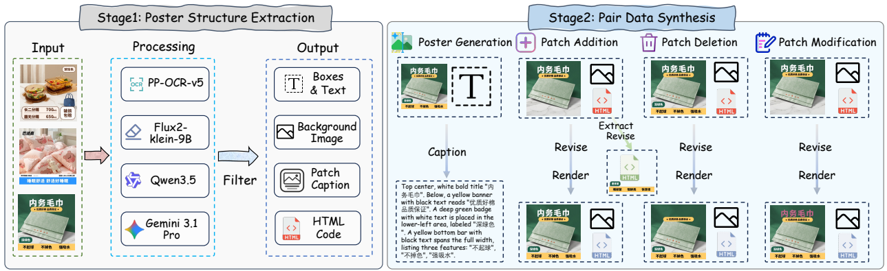
Figure 3: Overview of the data construction pipeline. The pipeline first extracts patch-level structural annotations from raw posters, and then constructs operation pairs for generation, addition, deletion, and modification.
