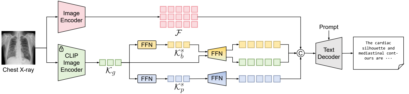
Fig. 4. Overview of EMGKT during inference phase.
