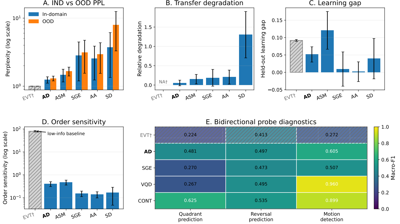
Figure 1. Transfer and structure across gaze representations on the bidirectional AEA↔RITW benchmark. Panels A–D summarize the hand-designed tokenizer comparison. Panel E shows the matched context-16 probe rerun with source-specific K = 128 VQD and CONT. EVT† uses AEA→RITW only in Panels A, C, and D. Panel B is NA because the RITW→AEA stream collapses to one deterministic token, making bidirectional degradation undefined. Abbreviations follow Sec. 3.2.
