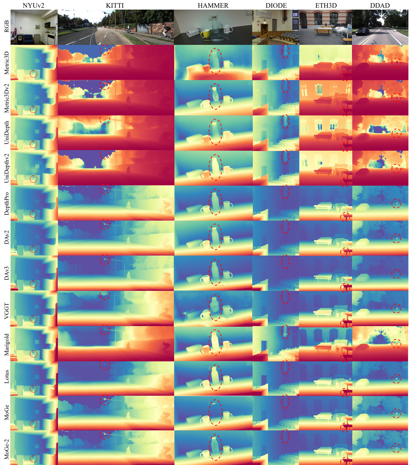
Fig. 7 Qualitative visualization of depth estimation results from representative models [18–21, 24, 25, 27–29, 32, 42, 43] across diverse scenarios, including indoor [12, 78], outdoor [79], driving [13, 81], and object-level scenes [76]. Despite some methods showed strong quantitative results, discrepancies remain between numerical performance and visual quality, particularly regarding boundary sharpness and detail preservation.
