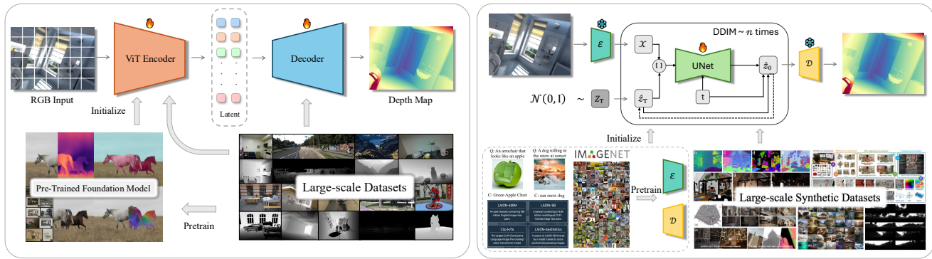
Fig. 5 Illustration of discriminative (left) and generative (right) frameworks for monocular depth estimation. Discriminative methods typically leverage a Vision Transformer [160] (ViT) encoder initialized with a pre-trained foundation model (e.g., DINOv2 [157]) and trained on large-scale diverse datasets to directly regress depth maps. In contrast, generative methods utilize VAE [161] structure, iteratively refining depth predictions through a denoising process conditioned on synthetic datasets, thereby effectively capturing complex details and structural coherence.
