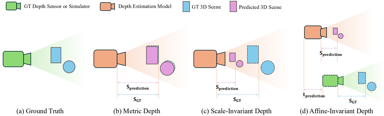
Fig. 2 Illustration of different depth estimation paradigms: (a) Ground-truth depth acquired from a depth sensor or simulator; (b) Metric depth estimation, the predicted depth is consistent with the ground truth in physical units; (c) Scale-invariant depth estimation, the predicted depth differs from the ground truth by a global scaling factor; (d) Affine-invariant depth estimation, the predicted depth diverges from the ground truth by both a global scale and an additive translation.
