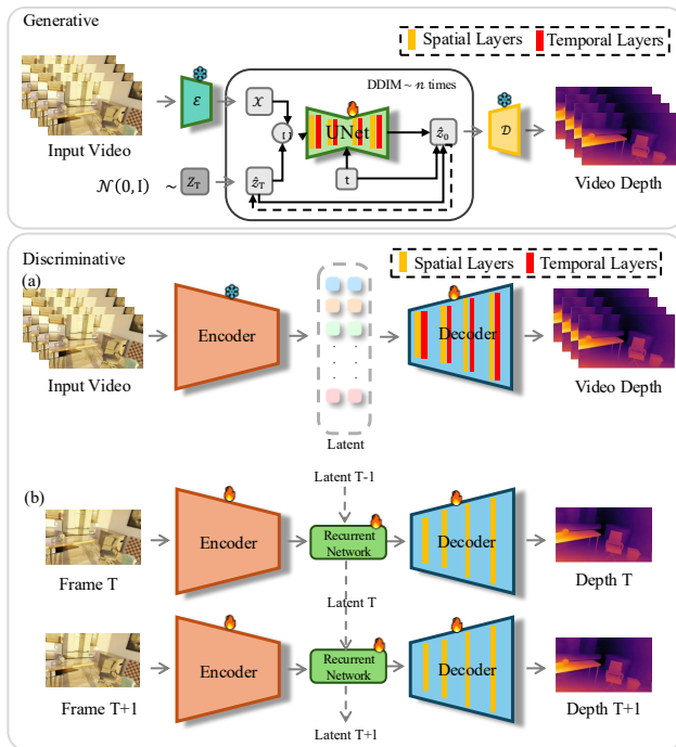
Fig. 8 Structure of video depth estimation. Unlike image depth estimation models, which use spatial layers to process each image, video depth estimation models additionally introduce temporal layers or utilize previous latent states via a recurrent neural network to ensure consistency across frames.
