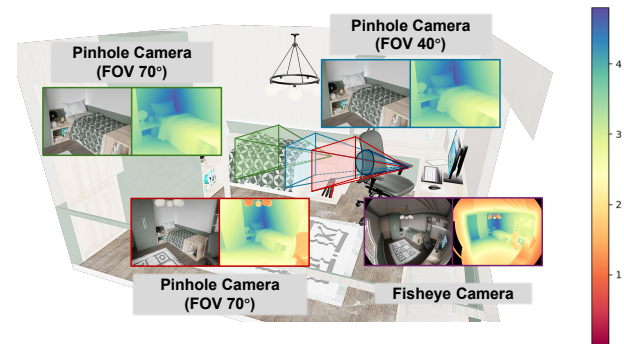
Fig. 6 Illustration of metric depth ambiguity across different camera models and intrinsics. We render the same indoor scene using four different cameras: three pinhole cameras (green, blue, red) with varying fields-of-view (FoV), and one fisheye camera (purple). Three cameras are placed at the same position (blue, red, purple), yet they produce significantly different appearance patterns due to variations in camera intrinsics and distortion, despite sharing the same underlying geometry. In contrast, pinhole cameras with different FoVs (green vs. blue) produce visually similar images but correspond to different depth distributions.
