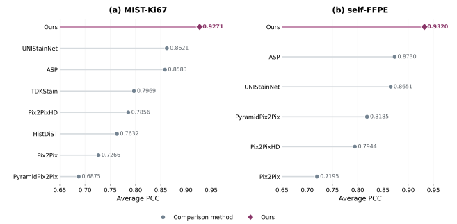
Fig. 6. Average PCC between generated images and their corresponding source images on the MIST-Ki67 and self-FFPE datasets. Higher values indicate stronger preservation of source-tissue organization.
