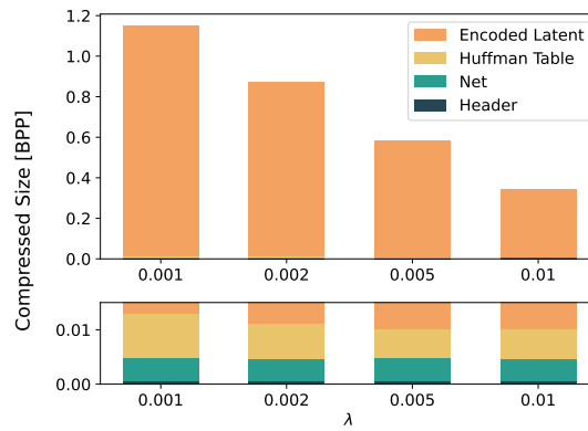
Fig. 12: Bitstream breakdown.
