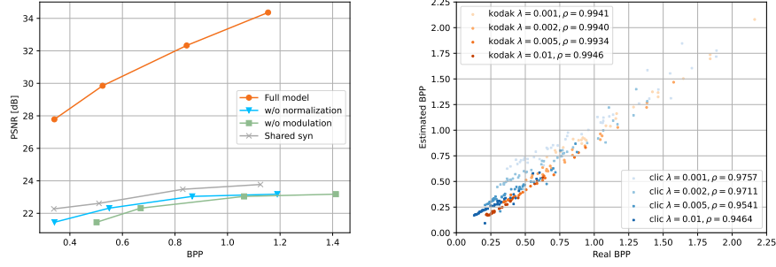
(a) Ablation of synthesis net g_s architecture. All components are necessary for performance. (b) Ablation of entropy model. \rho is Pearson correlation coefficient.
