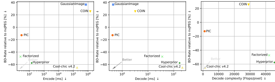
Fig. 8: Results of comprehensive comparison for both RD performance and practical performance on Kodak dataset.
