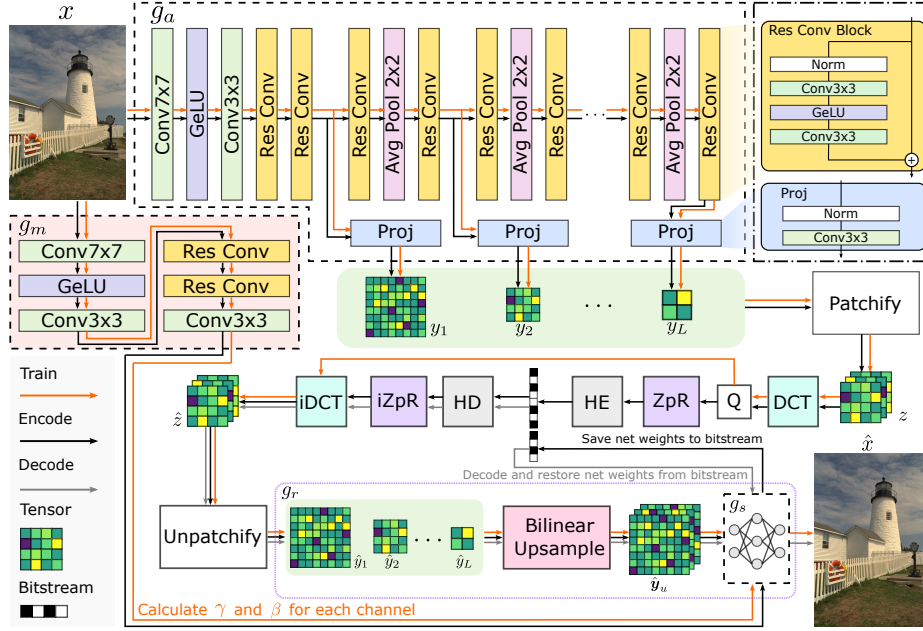
Fig. 1: The framework of PIC. The overall data flow is presented in an S-shaped in the diagram, following g_a \rightarrow \hat{\mathbf{y}} \rightarrow \mathbf{z} \rightarrow \hat{\mathbf{z}} \rightarrow g_r \rightarrow g_s . g_a and g_m are latent encoder and modulation net respectively. \hat{\mathbf{y}} = \{y_1, y_2, \dots, y_L\} are latents generated by latent encoder g_a . All latents are divided into patches of size 8 \times 8 and then concatenated together as \mathbf{z} . Similar to other compression methods, \mathbf{z} is quantized after DCT transformation. The ZpR module converts the quantized symbols into a more compact form, and we will discuss this module in detail in the Sec. 3.3. HE and HD are Huffman encoder and decoder. iZpR and iDCT are inverse transformation of DCT and ZpR respectively. g_r is part of the decoder and also acts as an image representation model. g_s is synthesis network. \gamma and \beta are mean and standard deviation of each channel of g_m output respectively.
