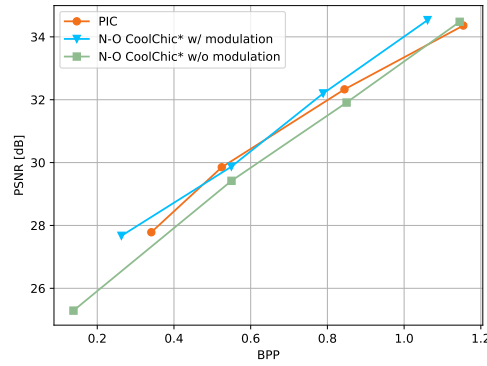
Fig. 11: Ablation results of modulation mechanism on N-O Cool-Chic-like (mark by *) architecture [5]. It should also be noted that N-O Cool-Chic is not open-source, so the results presented here are only a preliminary reproduction without hyperparameters and training receipts tuning and may differ from those reported in the original paper.
