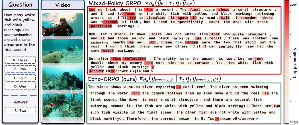
Figure 1: Reasoning in the words you know. Token-level log-probabilities under the policy \pi_\theta (red shading indicates low probability). Top: Mixed-Policy GRPO forces the policy to imitate privileged reasoning traces from a stronger teacher, leaving semantically critical ones, such as “school of fish,” in low-likelihood regions. Bottom: Echo-GRPO paraphrases the same reasoning into the policy’s native distribution (“school of fish” \rightarrow “several fish”), preserving the semantics while keeping all tokens within the policy’s distribution.
