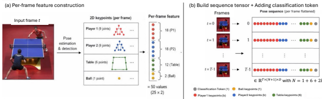
Figure 3: Construction of the input representation. (a) Keypoints from both players, the table, and the ball are extracted and concatenated. Here, 9 per player, 6 for the table, and 1 for the ball, resulting in 25 (x, y) keypoint coordinates per frame. (b) EventNet input by assembling the pose sequence across frames (projection each keypoint to size D ) and adding the CLS token of size D to each frame.
