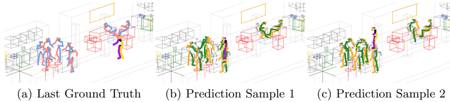
Fig. S5: Qualitative comparison on the HiK dataset (10-second prediction). We visualize two stochastic samples for the same scene. (a) Last observed GT at t = 2 s (frame 49). (b - c) Final predicted frame at t = 12 s (frame 299) from two distinct generated samples. Visualization scheme follows Fig. S1. The purple/yellow person walks to different locations in (b) and (c). This demonstrates the model’s ability to generate diverse predictions.
