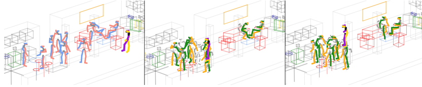
Fig. 3: Qualitative examples of 10-second predictions for the HiK dataset. We visualize two generated samples for the same input. We show the last observed frame on the left, followed by the final predicted frame from two distinct generated samples. These examples demonstrate the model’s ability to generate diverse predictions, as shown by the purple/yellow person walking to different locations.
