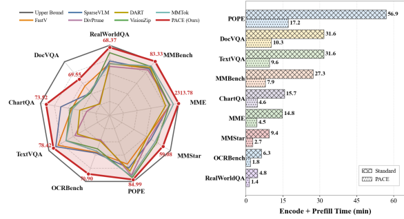
Figure 1: Accuracy–TTFT trade-off at 10% visual-token retention. PACE preserves accuracy while reducing pre-generation latency on Qwen2.5-VL-7B; standard denotes Vanilla inference of the original model.
