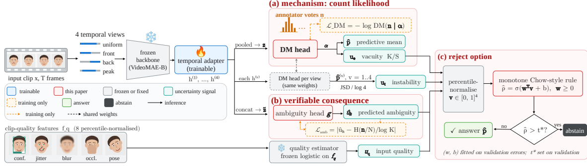
Fig. 2. Method overview, one row per inference-time signal. (a) The DM head maps the pooled \mathbf{z} to \alpha , giving \hat{\mathbf{p}} and the vacuity u_e ; applied to each \mathbf{h}^{(v)} it also gives the per-view means whose generalised JSD is the instability u_t . (b) The ambiguity head g regresses \hat{u}_h from \hat{\mathbf{z}} ; a frozen logistic estimator maps clip-quality features to u_q . (c) The four signals are percentile-normalised and fused by a monotone Chow-style rule with validation-chosen t^* . Votes \mathbf{n} enter only through the dashed training-only terms. Red outlines: components introduced here.
