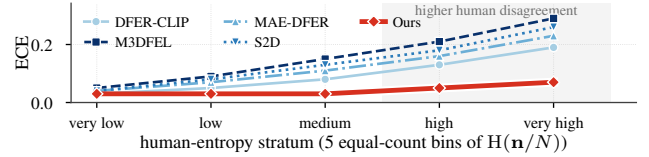
Fig. 1. Entropy-stratified ECE of four public DFER checkpoints on DFEW. Calibration degrades as human disagreement increases, with the largest overconfidence observed on the highest-entropy clips.
