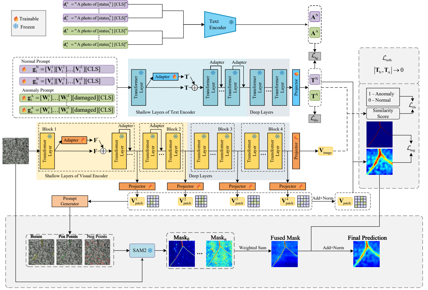
Fig. 1. Overview of the proposed PSMP-CLIP network. PPSS enables SAM2 to produce precise boundary segmentations and MSGPR preserves CLIP’s general knowledge and enriches task-specific semantics.
