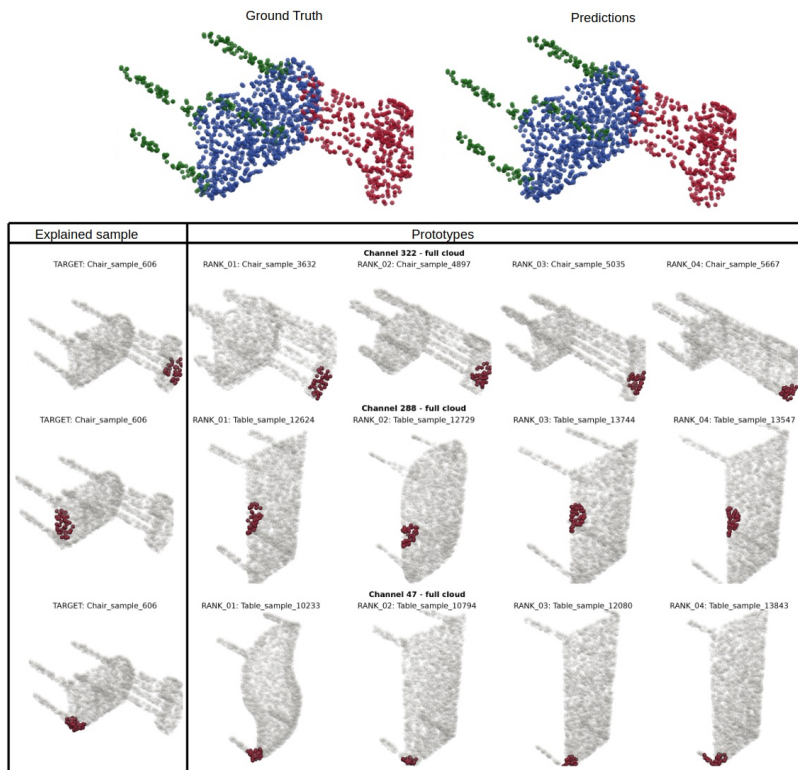
Figure 22: Explanation of the chair object from the ShapeNetPart dataset
