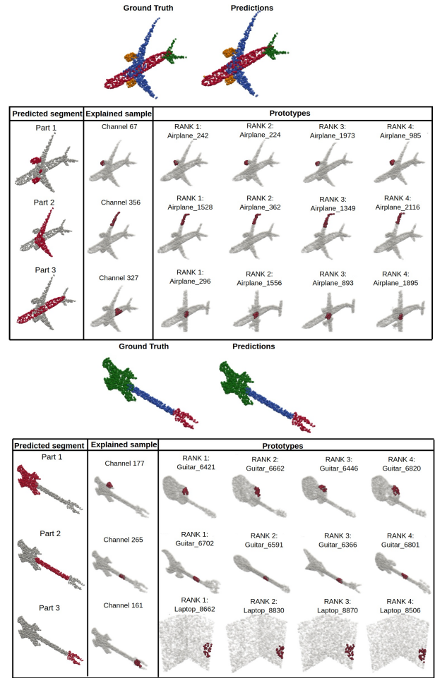
Figure 5: Examples of a PiPS explanation for point cloud data. For each predicted part class (first column) of the explained object, we select the patch with the most active channel (second column) that belongs to the corresponding segment. We then select prototypes from other objects for which the same channel is the most active (third column).
