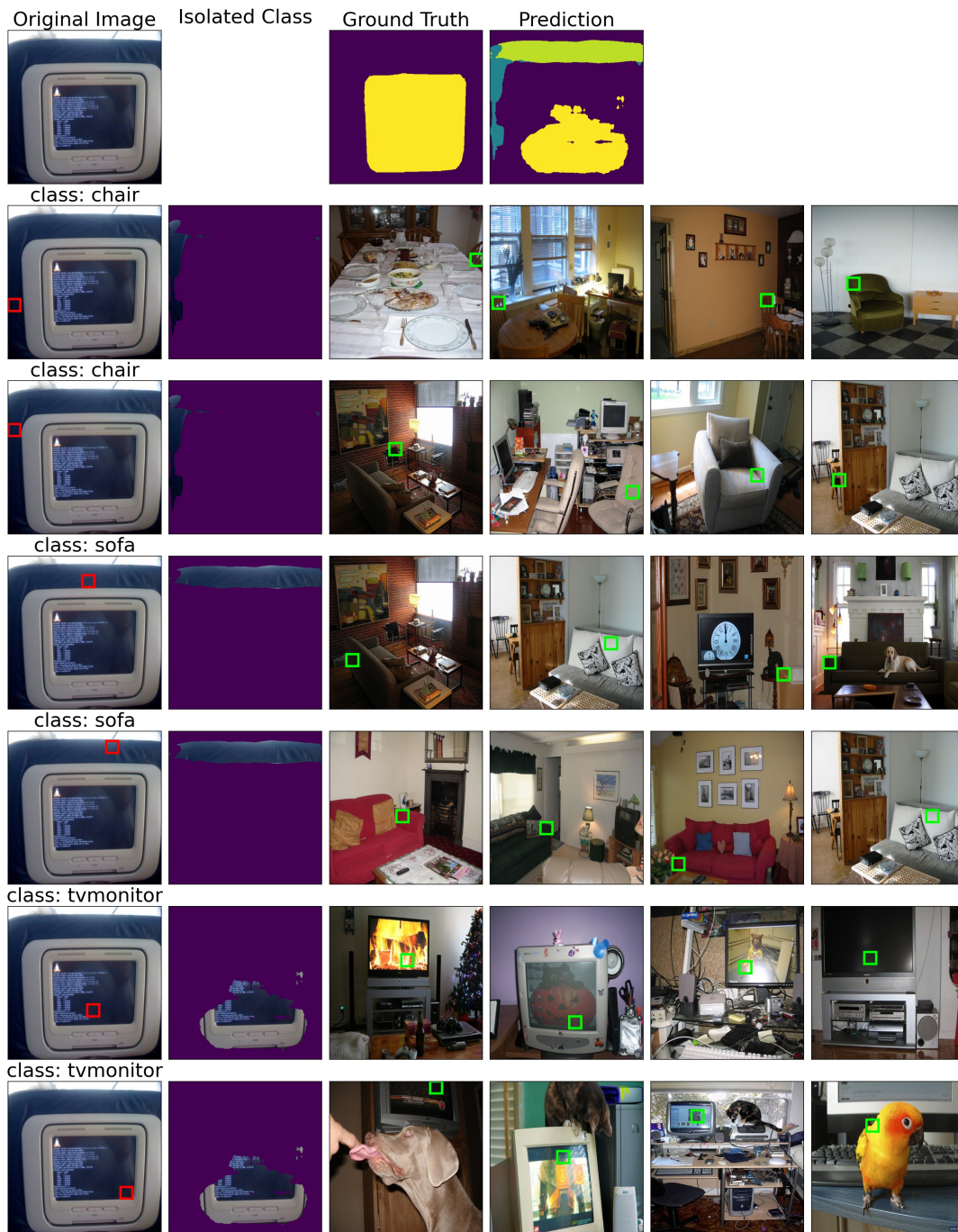
Figure 14: Visual explanation for the 'chair', 'sofa' and 'tvmonitor' objects identified during semantic segmentation
