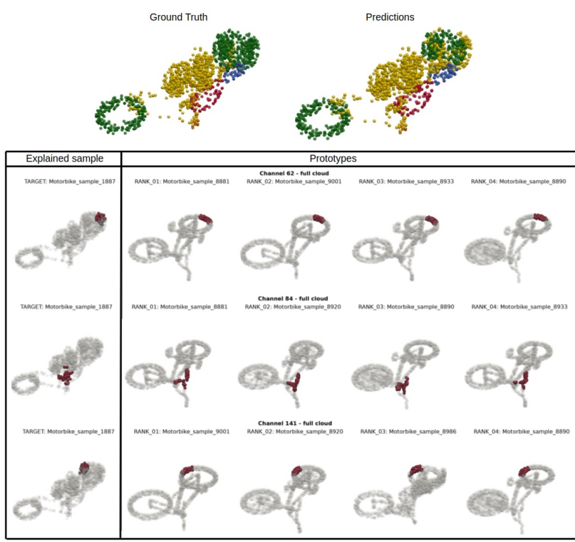
Figure 18: Explanation of the motor object from the ShapeNetPart dataset
