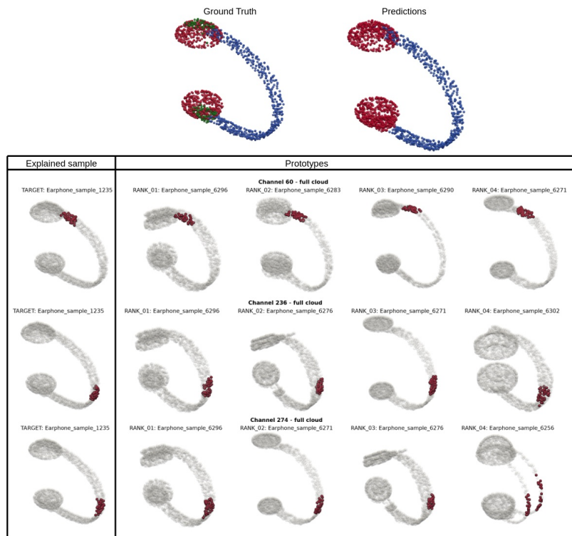
Figure 21: Explanation of the earphone object from the ShapeNetPart dataset
