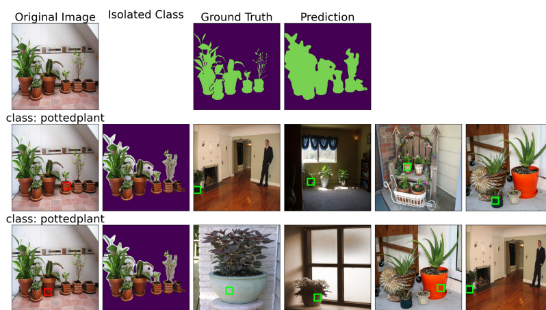
Figure 10: Visual explanation for the 'pottedplant' object identified during semantic segmentation
