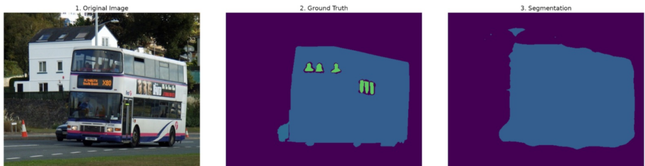
Figure 29: Segmentation quality comparison interface. In this task of the user study, participants were asked a question: “Which method generates a better segmentation?”. Users compared the spatial segmentation masks produced by PiPS against those generated by the ante-hoc ScaledProtoSeg method. For this comparison, participants could explicitly choose their preferred segmentation or select a neutral “Neither is better” option. Notably, SegGradCam was deliberately excluded from this specific task; because both PiPS and SegGradCam are strictly post-hoc methods operating on the identical frozen DeepLabV3 backbone, they inherently yield the exact same categorical segmentation outputs. Thus, this task effectively evaluated the visual quality of our perfectly preserved baseline predictions against the altered masks produced by the ante-hoc architecture.
