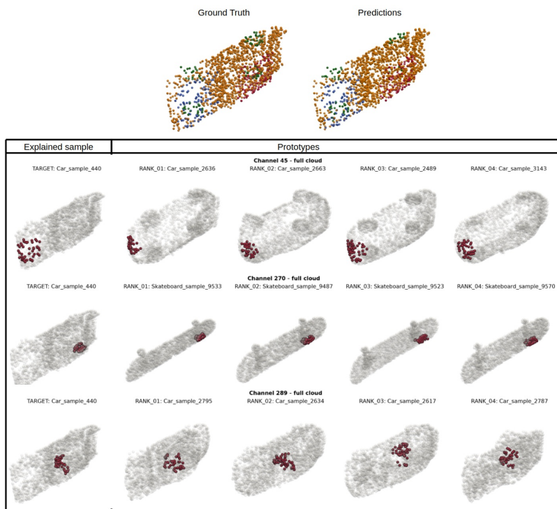
Figure 26: Explanation of the car object from the ShapeNetPart dataset
