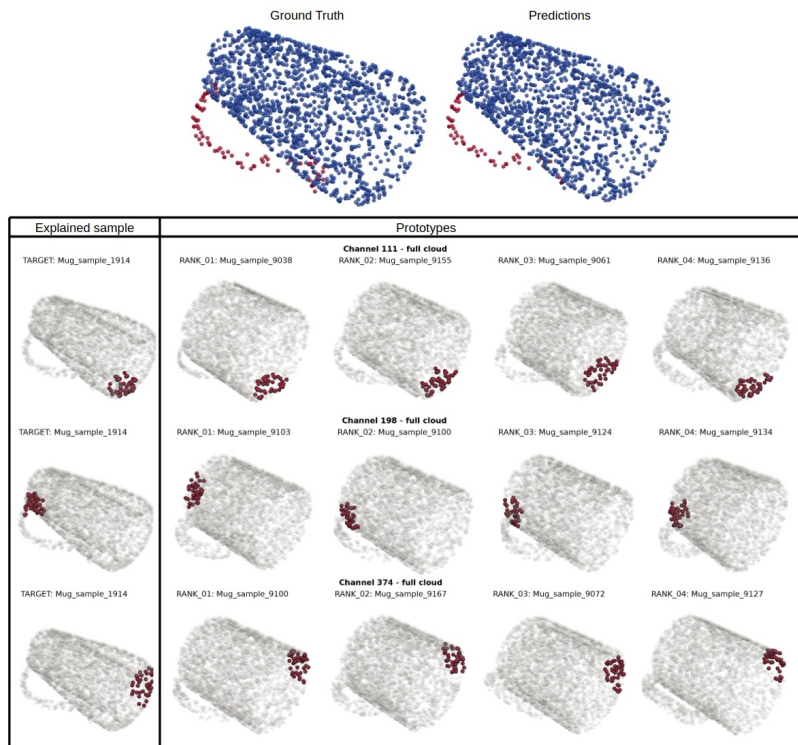
Figure 20: Explanation of the mug object from the ShapeNetPart dataset
