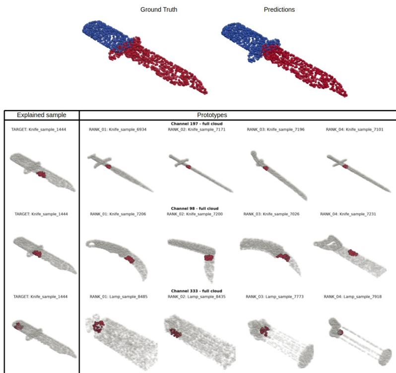
Figure 25: Explanation of the knife object from the ShapeNetPart dataset
