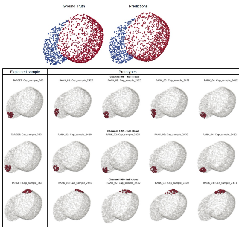
Figure 27: Explanation of the cap object from the ShapeNetPart dataset
