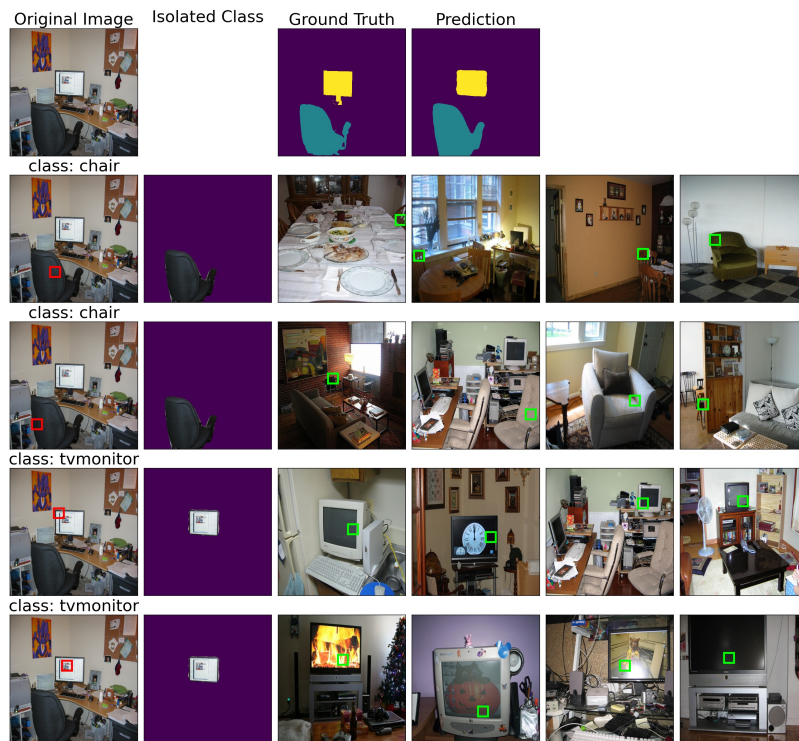
Figure 12: Visual explanation for the 'chair' and 'tvmonitor' objects identified during semantic segmentation
