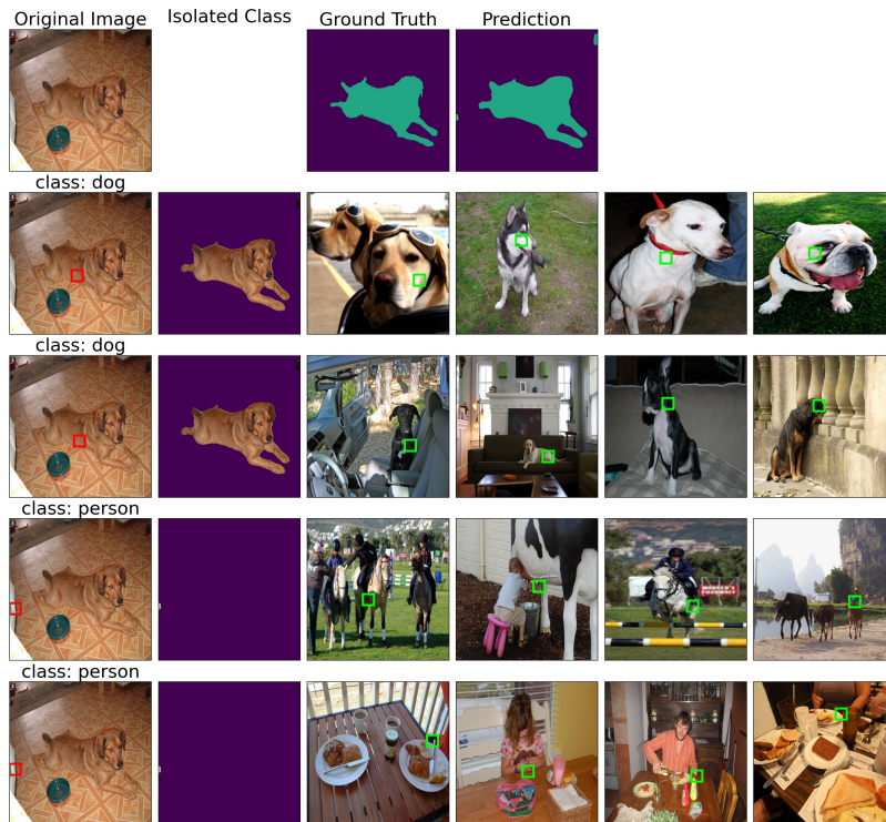
Figure 11: Visual explanation for the 'dog' and 'pearson' objects identified during semantic segmentation
