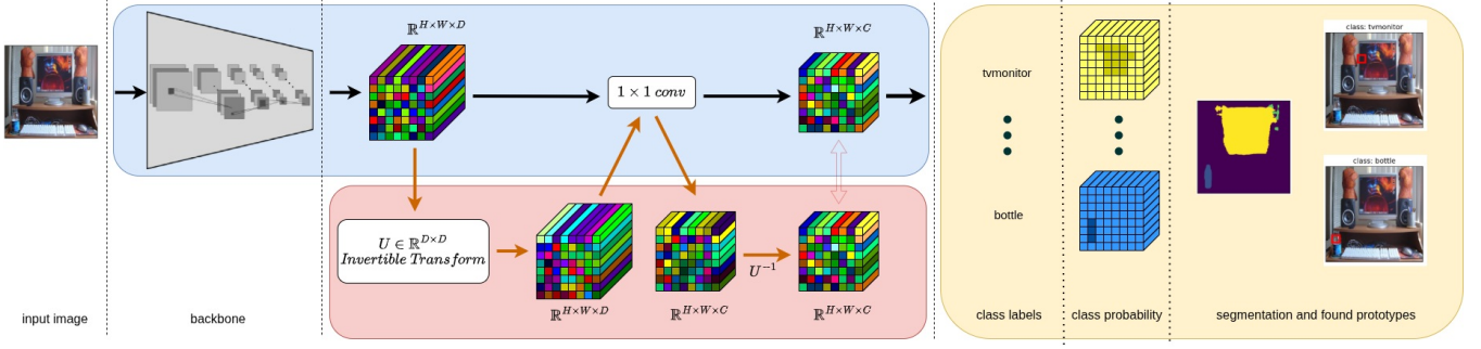
Figure 3: Overview of the PiPS training framework. The pre-trained backbone features are passed through a trainable invertible transformation matrix. We optimize a purity objective to isolate localized concepts. During training, we dynamically subset the dataset based on exemplar scores to progressively focus on the most representative prototypes.
