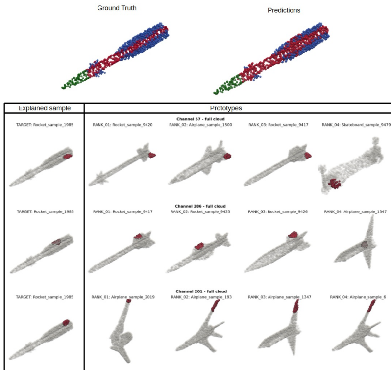
Figure 19: Explanation of the rocket object from the ShapeNetPart dataset
