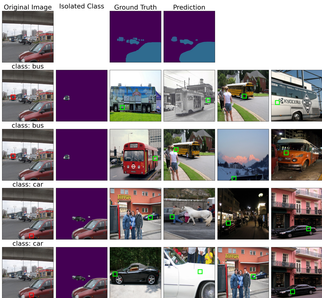
Figure 13: Visual explanation for the 'bus' and 'car' objects identified during semantic segmentation
