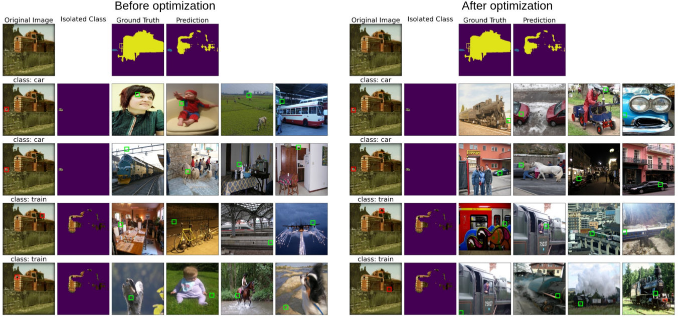
Figure 4: Impact of the optimization phase on the generated explanations. Visual comparison of the extracted prototypical parts before (left) and after (right) the purity-driven optimization process on the pre-trained segmentation backbone. As observed, prototypes without the additional tuning correspond to random, uninterpretable image patches with limited explanatory properties. After the optimization, these prototypes become highly consistent and accurately correspond with the localized semantic features of the input image.
