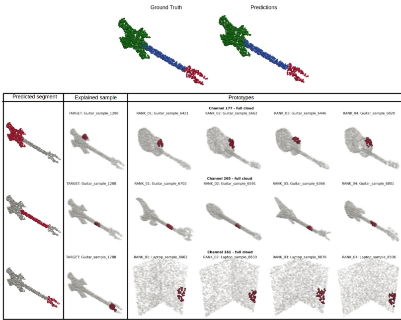
Figure 17: Explanation of the guitar object from the ShapeNetPart dataset
