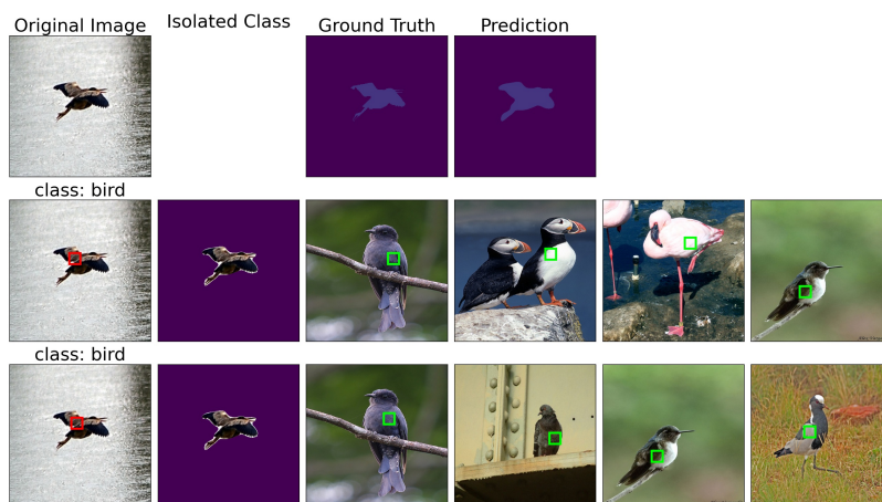
Figure 8: Visual explanation for the 'bird' object identified during semantic segmentation
