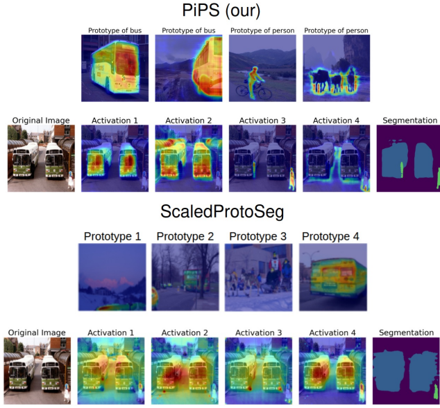
Figure 2: Comparison of PiPS and ScaledProtoSeg with heatmaps. Visual evaluation using heatmaps illustrating the spatial activation patterns and localization performance of prototypical parts generated by PiPS and ScaledProtoSeg on semantic segmentation tasks. Notice the variations in activation in compared approaches.
