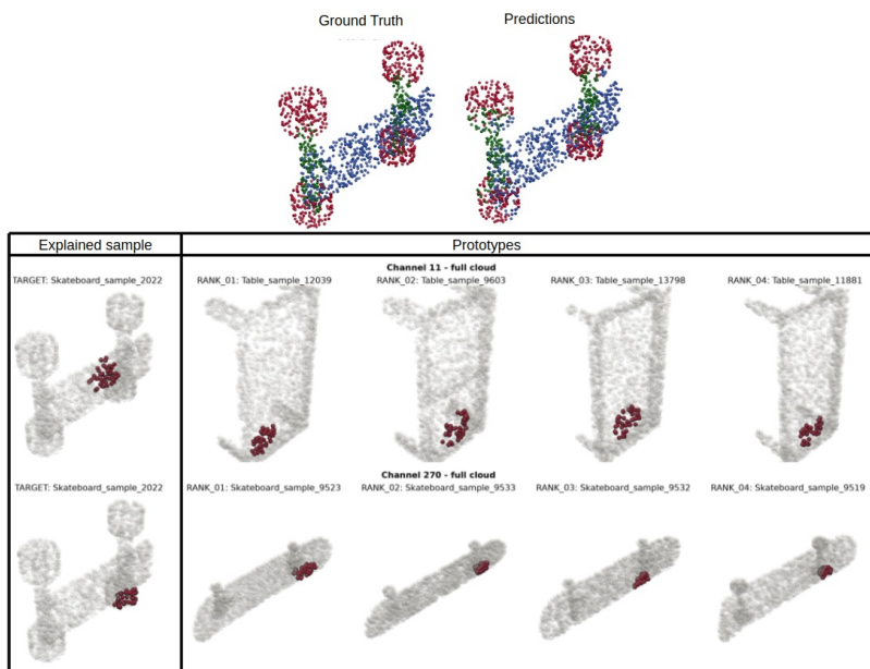
Figure 24: Explanation of the skateboard object from the ShapeNetPart dataset
