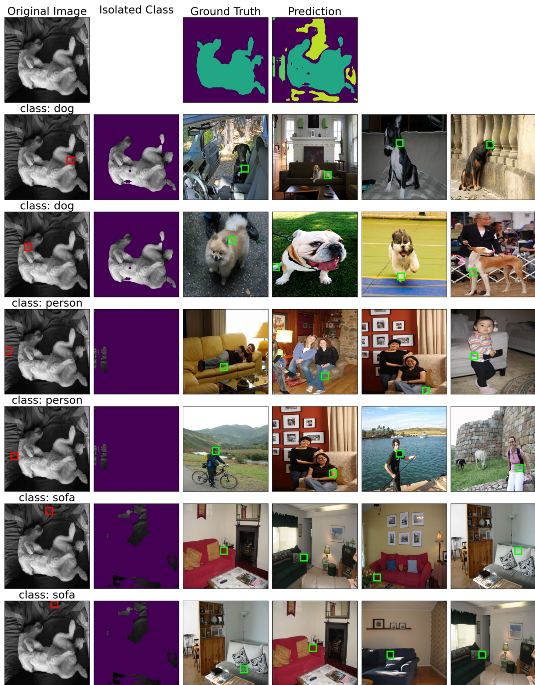
Figure 15: Visual explanation for the 'dog', 'person' and 'sofa' objects identified during semantic segmentation
