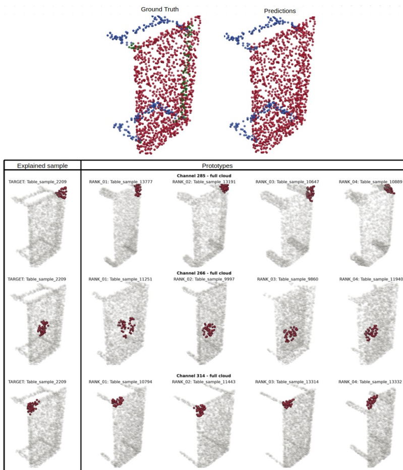
Figure 23: Explanation of the table object from the ShapeNetPart dataset
