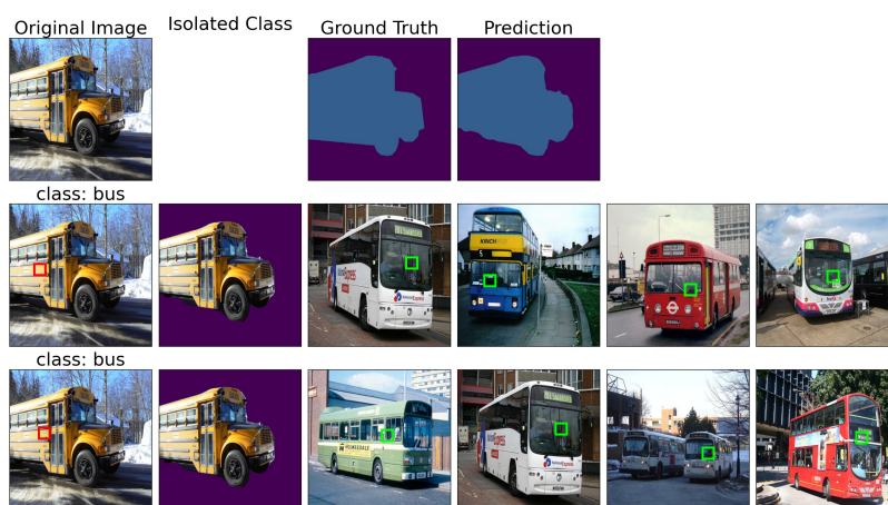
Figure 9: Visual explanation for the 'bus' object identified during semantic segmentation
