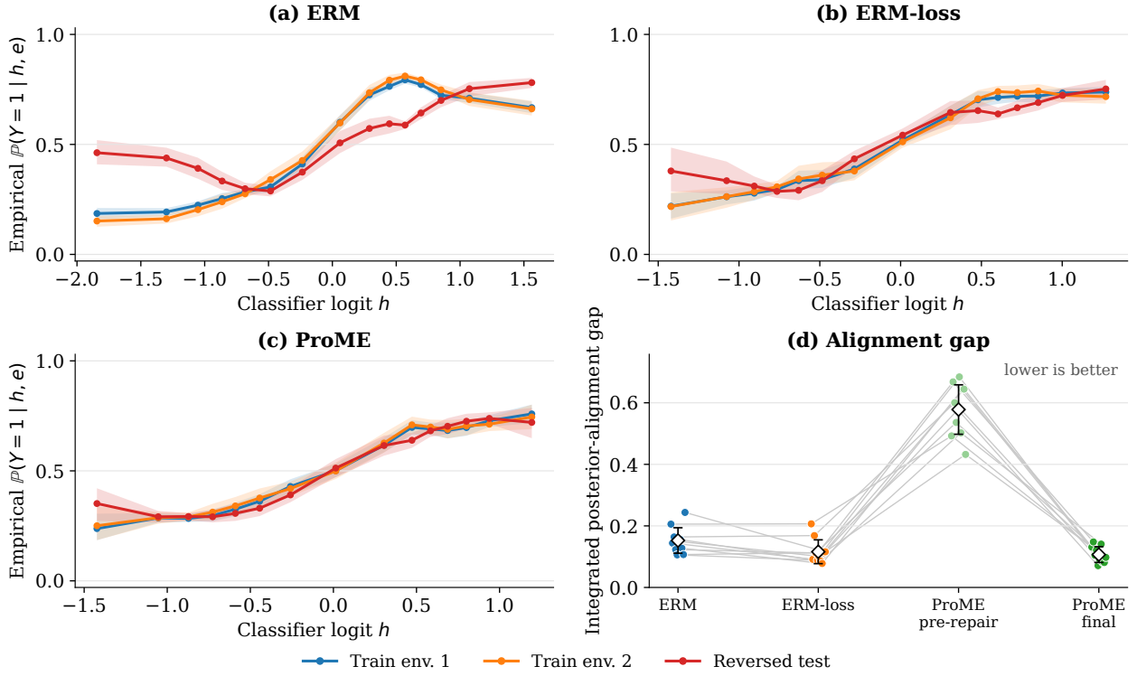
Fig. 6. Classifier repair reduces the posterior-alignment gap on ColoredMNIST. Panels (a)–(c) plot the empirical \mathbb{P}(y=1 | h, e) for two training environments and the reversed test environment under ERM, ERM-loss, and ProME after classifier repair. Panel (d) reports the integrated posterior-alignment gap for ERM, ERM-loss, and ProME before and after repair. A lower value indicates better alignment. Gray lines connect the same seed. Curves use 50 equal-width bins with at least five samples per bin.
