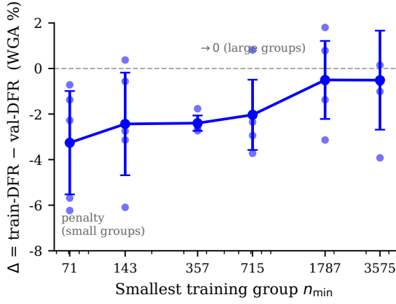
Fig. 8. Effect of minority support on classifier-repair label source. train-DFR minus val-DFR WGA versus the smallest training group n_{\min} , reported as mean \pm standard deviation over five seeds.
