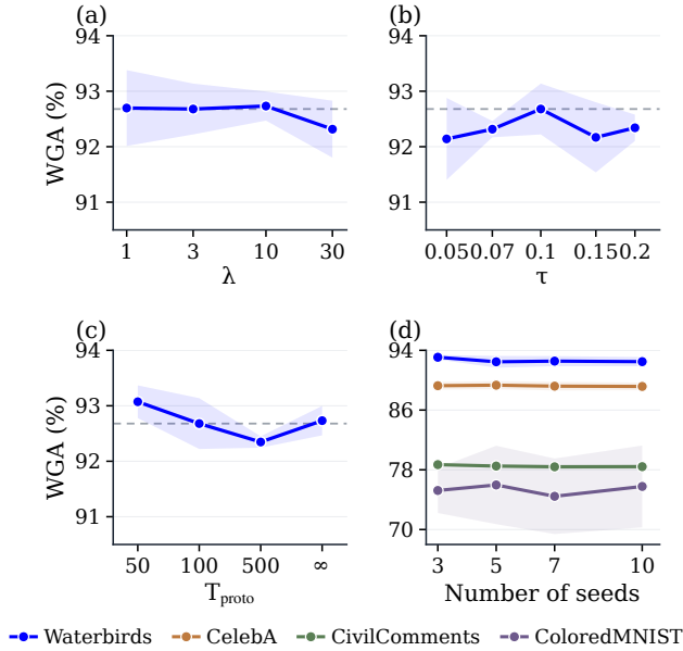
Fig. 9. Hyperparameter and seed-budget sensitivity. (a–c) Label-augmented Waterbirds diagnostic across the invariance weight, temperature, and prototype-refresh period; bands show standard deviations and dashed lines mark defaults. (d) WGA across seed budgets.
