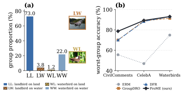
Fig. 1. Training-group imbalance and worst-group accuracy. (a) Group proportions in the Waterbirds training set. (b) Reported WGA of representative methods, including deep feature
