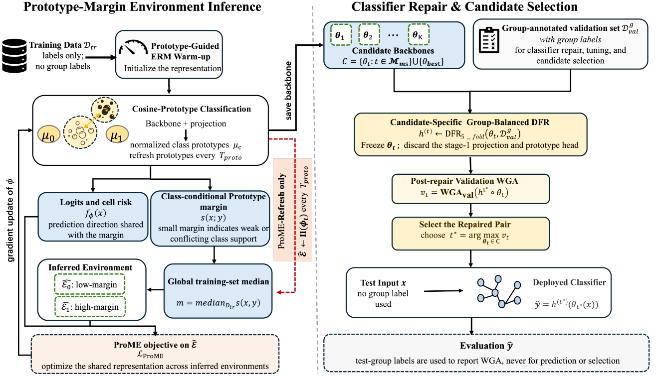
Fig. 2. Overview of ProME. Stage 1 learns representation candidates from prototype-margin environments without training-group labels. Stage 2 repairs and selects candidates using group-annotated validation data, with five-fold cross-validation for regularization tuning. The dashed path denotes ProME-Refresh.
