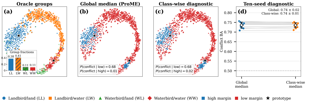
Fig. 3. Prototype-margin enrichment of shortcut conflicts on Waterbirds. Panels (a–c) show the same seed-42 test examples in a shared t-distributed stochastic neighbor embedding (t-SNE). (a) Oracle groups; the inset reports their fractions in the displayed subset. (b) Environments induced by the global-median rule used by ProME. (c) Environments induced by a class-wise median diagnostic. Marker shapes denote oracle groups, colors denote inferred environments, and stars denote class prototypes. (d) Conflict balanced accuracy on the training split over ten seeds. Gray lines connect the same seed; diamonds and error bars show the mean and standard deviation.
