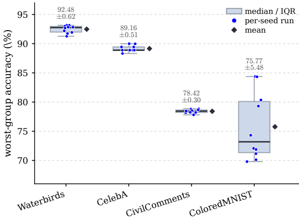
Fig. 7. WGA across ten fixed seeds. Boxes show interquartile ranges, center lines show medians, points show individual runs, and diamonds show means.
