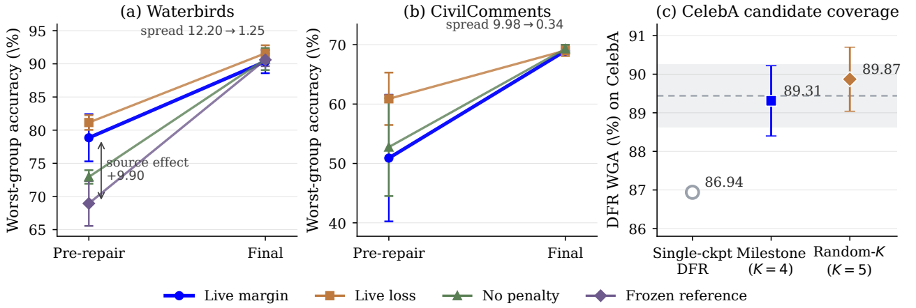
Fig. 5. Repair-aware candidate evaluation. (a) Waterbirds and (b) CivilComments before and after classifier repair; each line connects one Stage 1 variant of Table 4. (c) CelebA with single-checkpoint, milestone, and random candidate sets under a fixed repair procedure; the band marks the full multi-candidate pipeline.
