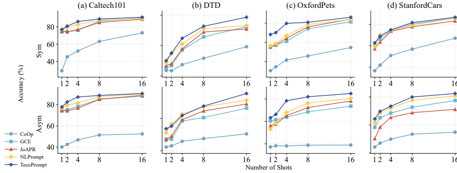
Fig. 4: Few-shot robustness under label noise with different shot budgets. We vary the number of shots per class over 1, 2, 4, 8, 16, while keeping the noise rate at 50%.
