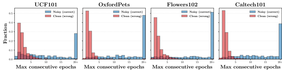
Fig. 1: Distribution of the maximum number of consecutive epochs during which the OT pseudo-label remains unchanged. For noisy examples, we count runs in which the stable OT label matches the ground-truth (Noisy, correct); for clean examples, we count runs in which the stable OT label is incorrect (Clean, wrong). Across datasets, noisy examples frequently exhibit long stable-correct runs (including the “20+” bin), whereas clean examples rarely sustain long stable-wrong runs.
