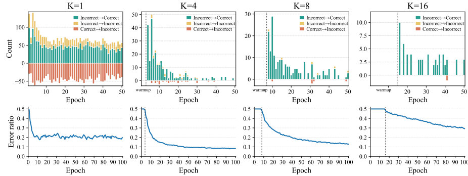
Fig. 5: Effect of the temporal stability window size K for conservative hard label rewriting. The top row reports the per-epoch counts of rewriting outcomes, including incorrect→correct, incorrect→incorrect, and correct→incorrect. The bottom row shows the ratio of incorrect labels in the dataset over training. The dashed line denotes the warm-up stage before rewriting is enabled.
