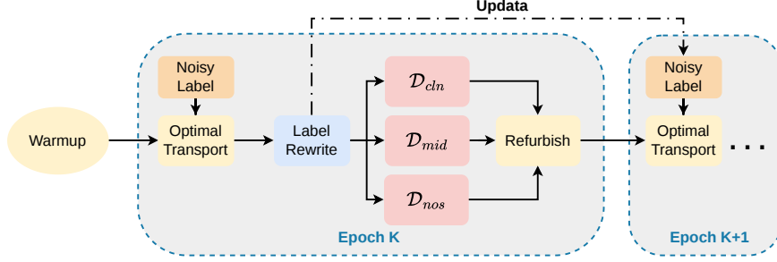
Fig. 3: Optimal Transport generates pseudo-label candidates to rewrite noisy annotations. Through iterative updates over epochs, incorrect labels are progressively corrected, reducing the noise rate and improving the quality of supervision.
