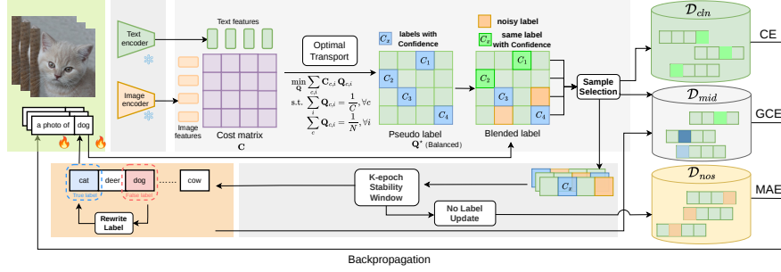
Fig. 2: Overview of the proposed TecoPrompt framework. Given frozen CLIP image/text encoders, we compute image embeddings and prompt-conditioned text prototypes, and solve a balanced entropic optimal transport problem to obtain globally consistent pseudo-label distributions. We then blend the OT pseudo-labels with the observed noisy labels using confidence weighting (where confidence scores are EMA-smoothed), perform sample selection to form clean/mid/noisy groups, and optimize prompts with a tri-group objective. In parallel, we track the OT-induced label trajectory over epochs and apply EMA-gated temporal consistency with a K -epoch stability window to conservatively trigger hard-label rewriting, thereby forming a closed-loop refinement that mitigates confirmation bias.
