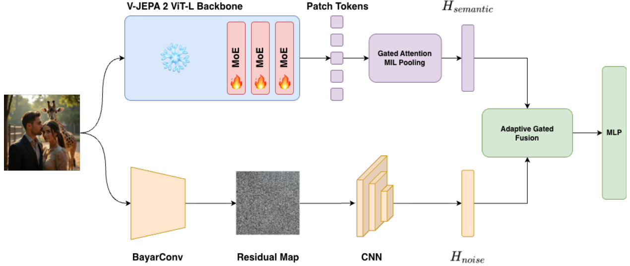
Figure 1. Overview of the MoE-JEPA architecture. The semantic branch (top) uses a V-JEPA 2 backbone, a MoE module, and a Gated Attention MIL module to semantically suppress pristine backgrounds and isolate localized tampering ( H_{\text{semantic}} ). In parallel, the noise branch (bottom) applies a constrained BayarConv layer to extract high-frequency generative and sensor artifacts ( H_{\text{noise}} ). These complementary features are joined using an Adaptive Gated Multimodal Fusion module and classified via an MLP head.
