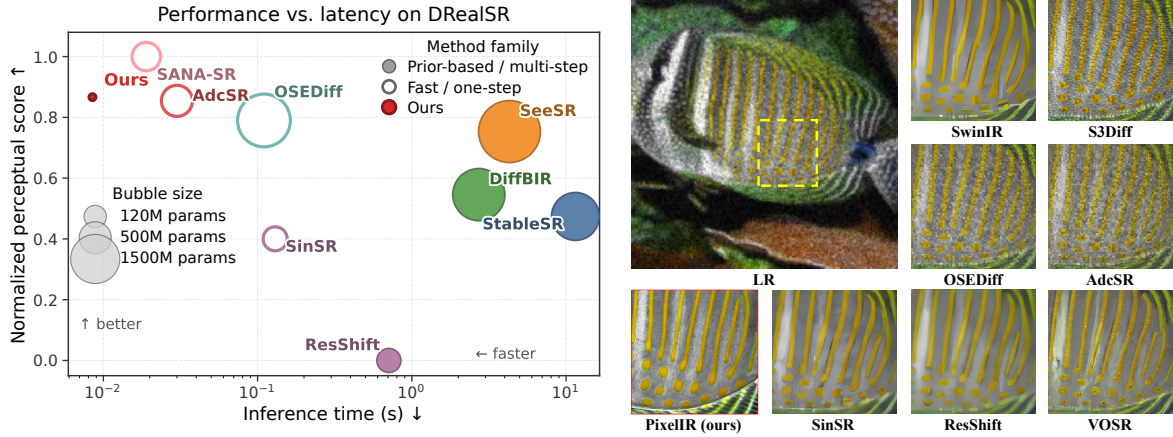
Figure 1: The compact PixelIR student achieves a favorable quality–efficiency trade-off for Real-ISR. Left: DRealSR perceptual score versus latency. Right: comparison against seven baselines.
