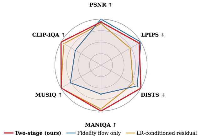
Figure 4: Six-metric component profile on DIV2K. Each metric is direction-aligned and normalized by its best value; farther is better.
