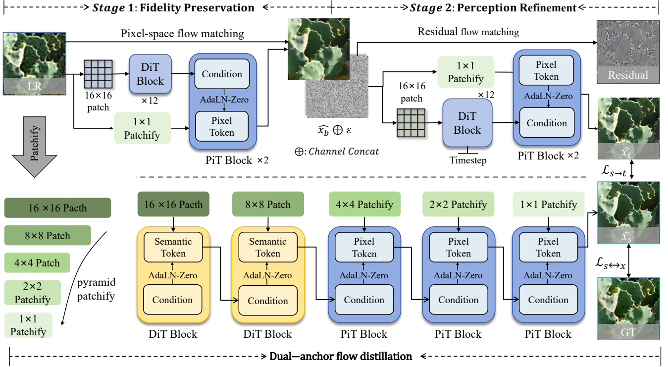
Figure 2: Overview of PixelIR. Given an upsampled LQ input, PixelIR first obtains a faithful base reconstruction \hat{x}_b with a 4-step image flow, then generates a complementary residual \hat{r} with a 4-step residual flow conditioned on the frozen base and forms the teacher output \hat{x}_t through residual composition. Both stages use a dual-granularity pixel transformer with semantic DiT and pixel-level PiT blocks. The teacher is further distilled into a progressively narrowed five-stage student \mathcal{S}_\phi , guided by the teacher anchor \mathcal{L}_{s \rightarrow t} and the bidirectional ground-truth anchors \mathcal{L}_{s \leftrightarrow x} for efficient one-step deployment.
