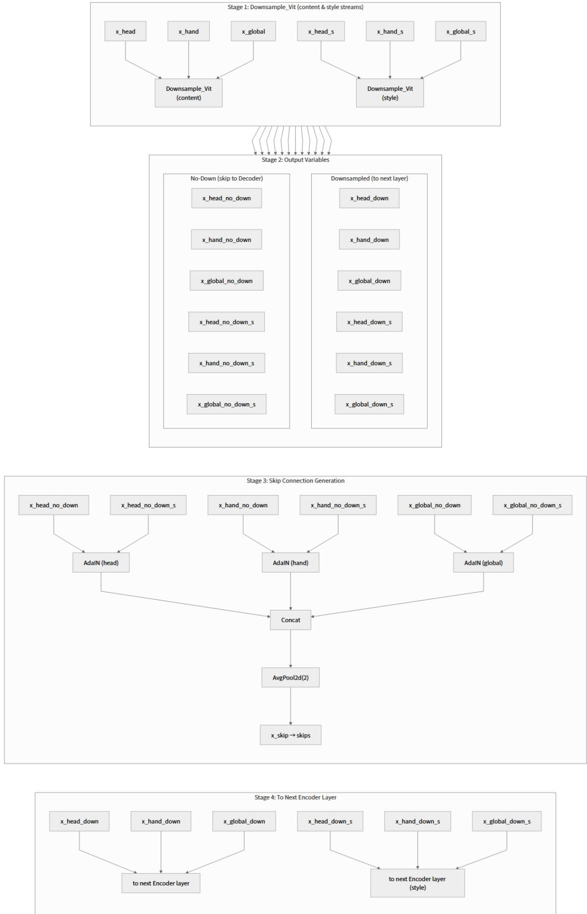
Figure 1: Encoder architecture with three parallel branches (head, hand, global). Each branch processes identical input through independent dual-pathway Downsample_Vit blocks. AdaIN fuses content and style streams at each level to produce skip connections.
