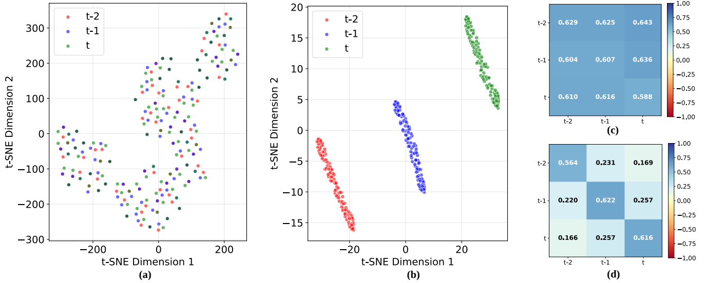
Fig. 7. Visualization of the Temporal Disentangling Net (TDN) ablation. The Key Point feature embeddings before (a) and after (b) passing through TDN from frames t - 2 , t - 1 , and t are projected into 2D using t-SNE and plotted as scatter plots, with colors indicating frame indices. Cosine similarities among the 3 frames' Key Point embeddings are also computed before (c) and after (d) TDN and visualized as heatmaps.
