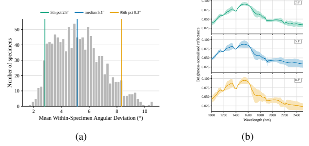
Fig. 2: Pixel-level spectral uniformity: (a) Distribution of the Mean Within-Specimen Angular Deviation (MWAD). (b) Mean spectra with corresponding spectral envelopes for representative specimens.
