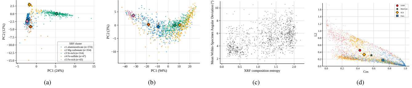
Fig. 3: (a) PCA projection of XRF composition vectors, grouped into five chemically coherent clusters. (b) PCA projection of the mean hyperspectral spectrum of each specimen, coloured according to the XRF-derived clusters in (a) (diamonds indicate cluster centroids of (a)). (c) MWAD and XRF composition entropy scatterplot. (d) Performance of our method and the baselines across all specimens, evaluated using the XRF measurements.
