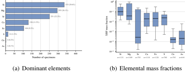
Fig. 1: XRF diversity: (a) Number of specimens for which an element is dominant. (b) Distribution of non-zero elemental mass fractions across specimens.
