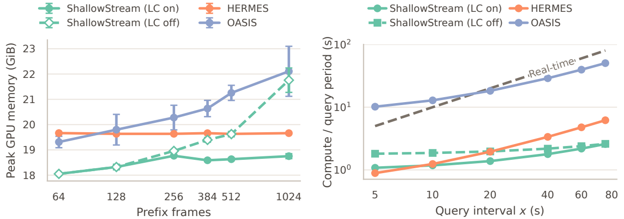
Figure 4 Continuous-stream memory and compute demand. Left: Peak GPU memory over lengths from 64 to 1,024 frames, averaged over five videos. Both variants use the final calibrated Gate and token-vote retriever. Right: For a query interval x , each curve combines mean query computation over the same five long-video cases with stream-time prefill accumulated over x seconds at 1 FPS. The dashed y = x boundary separates configurations that finish within the query interval (below) from those whose compute exceeds it (above).
