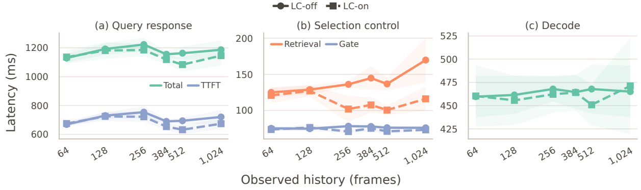
Figure 9 Query-time scaling on an NVIDIA RTX 5090. All six collected history lengths are shown. (a) Total query latency and time to first token (TTFT). (b) Evidence-selection and Gate latency. (c) Decoding latency. Solid circles denote full-history LC-off and dashed squares denote the matched final LC-on setting. Curves show means over five retrieval queries, and shaded regions denote 95% confidence intervals.
