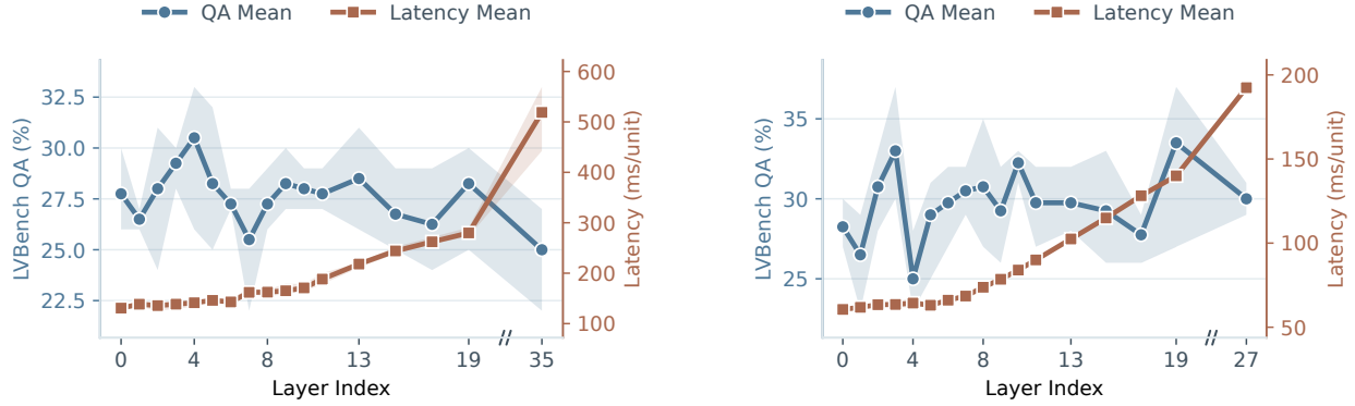
Figure 2 Layer-wise retrieval capability and stream-time prefill cost on LVBench. The left and right plots show results for Qwen3-VL-8B and LLaVA-OneVision-7B, respectively. We vary only the layer used for video-question matching. Latency is measured per video unit.
