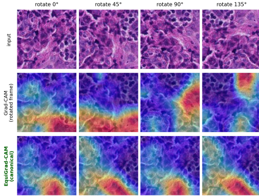
Figure 3. Explanation drift under rotation, histopathology. Each map is computed on the rotated input. Top : Grad-CAM, shown in the rotated frame, which drifts. Bottom : EquiGrad-CAM, inverse-rotated to the canonical frame, where an equivariant method yields the same map across the row.
