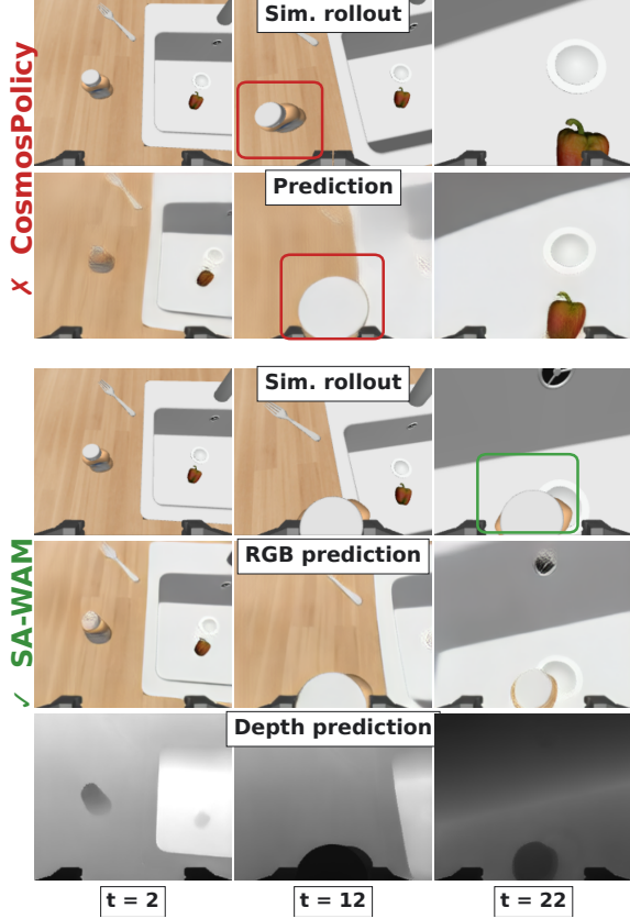
Fig. 3: RoboCasa pick-and-place task: Pick the condiment bottle from the counter and place it in the sink. We show the wrist view before and during grasping, and at the final rollout stage. The upper block shows Cosmos-Policy and the lower block shows SA-WAM, with predictions compared against their corresponding simulator rollouts; for SA-WAM we also show depth predictions. Red boxes mark rollout inconsistencies, and the green box marks task completion.
