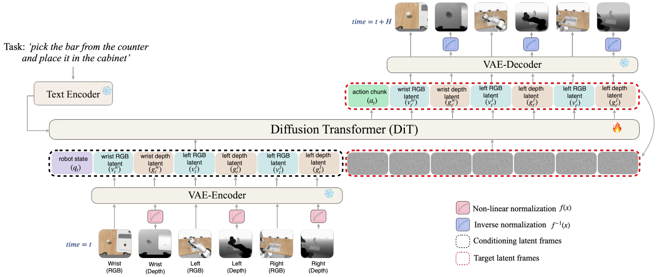
Fig. 2: SA-WAM architecture. SA-WAM injects geometry into the WAM latent sequence as tokenizer-compatible frames paired with each RGB view, while the proprioception ( q_t ) and action chunk ( a_t ) are inserted directly into dedicated positions in the latent sequence. The conditioning signals include the task description ( task ), one RGB frame per view ( v_t^c ) interleaved with its corresponding 3D modality ( g_t^c ) and the proprioceptive information at time t ( q_t ). The action chunk, future-state RGB ( v_t^c ), and future depth ( g_t^c ) frames undergo the denoising process. The decoding phase is optional at inference time.
