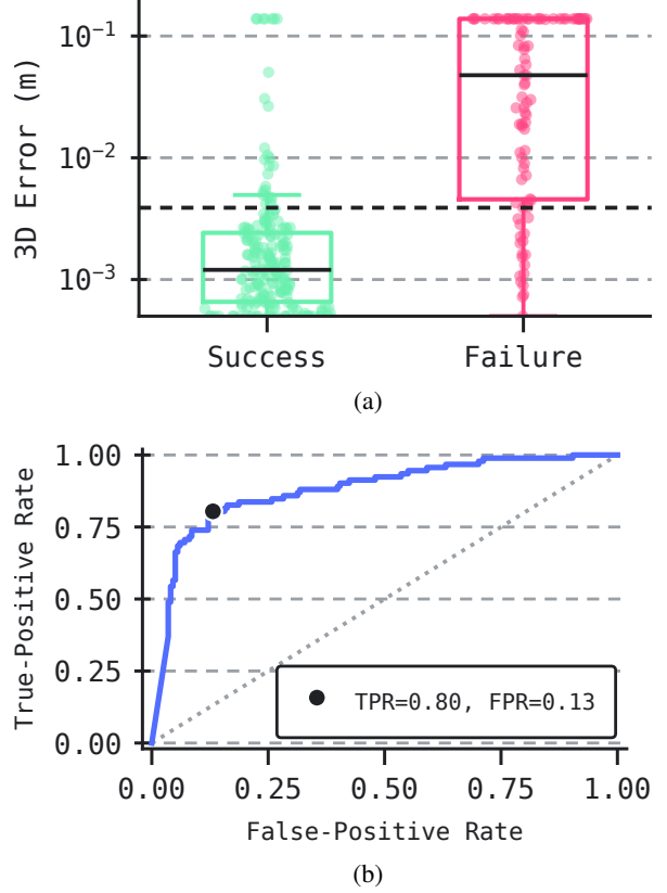
Fig. 4: Future-prediction quality correlates with rollout success. (4a) Object-centric 3D prediction error is lower for successful rollouts. (4b) A threshold on this error detects failures with AUC \approx 0.88 and an operating point of 80% detection at 13% false positive rate.
