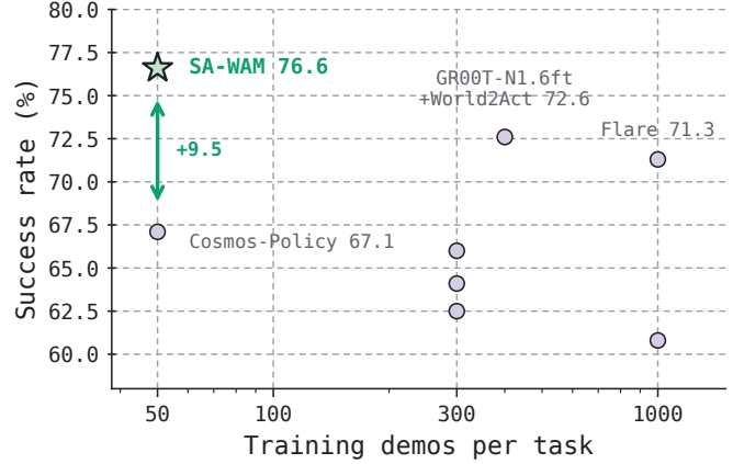
Fig. 1: State-of-the-art results on the RoboCasa benchmark. SA-WAM reaches 76.6% success rate on RoboCasa with only 50 demonstrations per task, improving over the matched Cosmos-Policy baseline by 9.5 points and outperforming prior approaches trained with 6–20× more data.
