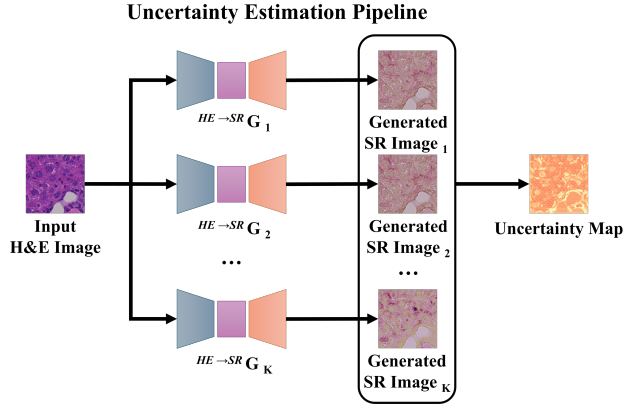
Figure S1: Epistemic uncertainty estimation via deep ensembles. An H&E input tile is forwarded through K=10 independently trained generators; the pixel-wise sample variance across the K SR outputs yields the uncertainty map \mathbf{U}(x) .
