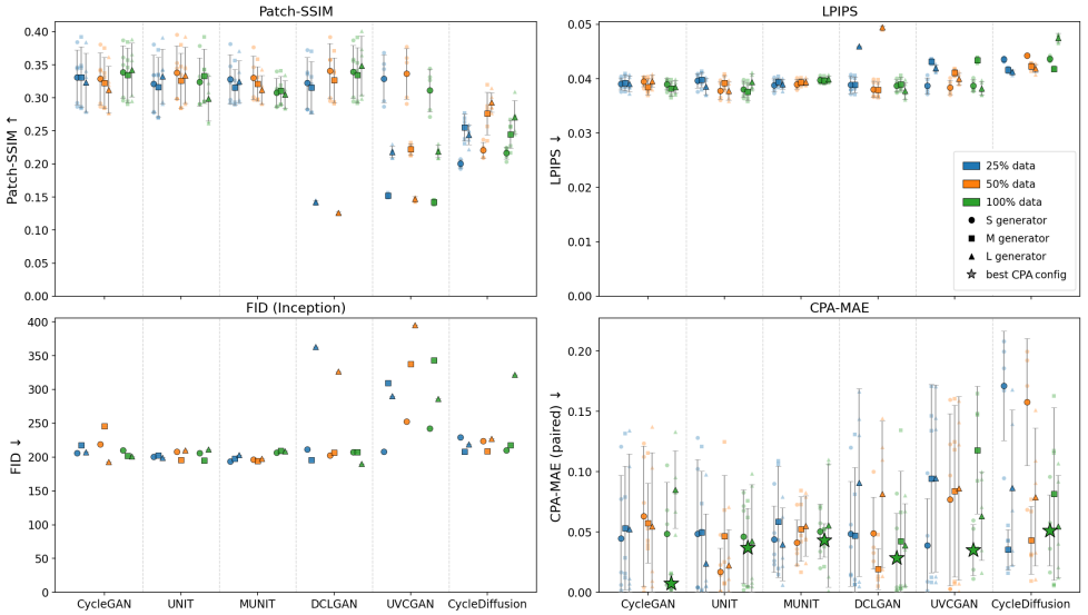
Figure 2: All four evaluation metrics across the 54 scaling configurations (6 models \times 3 sizes \times 3 data fractions). Colour encodes training data fraction (blue: 25%, orange: 50%, green: 100%); marker shape encodes generator size (circle: small S, square: medium M, triangle: large L). Large star markers indicate the best-performing model size at the 100% data fraction per model family, selected for ensemble uncertainty estimation in Section 6. Error bars on Patch-SSIM, LPIPS, and CPA MAE denote \pm std over N=5 held-out paired specimens (10 WSIs); FID is a set-level statistic with no per-sample variance. Vertical axis directions: Patch-SSIM higher is better; LPIPS, FID, CPA MAE lower is better.
