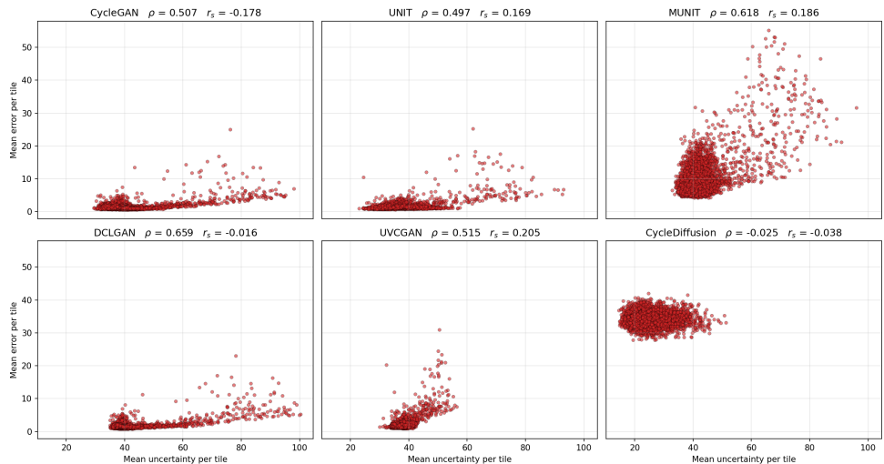
Figure S4: Across-tile scatter plots of tile-mean uncertainty \bar{U} ( x -axis) versus tile-mean cycle-reconstruction error \bar{E} ( y -axis) for each model family (top row: CycleGAN, UNIT, MUNIT; bottom row: DCLGAN, UVCGAN, CycleDiffusion). Uncertainty is on the same linear 0–255 intensity scale as the per-tile \bar{\sigma} of Figure 4 in the main paper. Pearson \rho and Spearman r_s are annotated per panel. GAN-based families show moderate Pearson correlations (0.50–0.66) driven by high-leverage tiles at large uncertainty values; Spearman correlations are substantially weaker, indicating the relationship is non-monotonic. CycleDiffusion (bottom right) shows no meaningful correlation in either metric.
