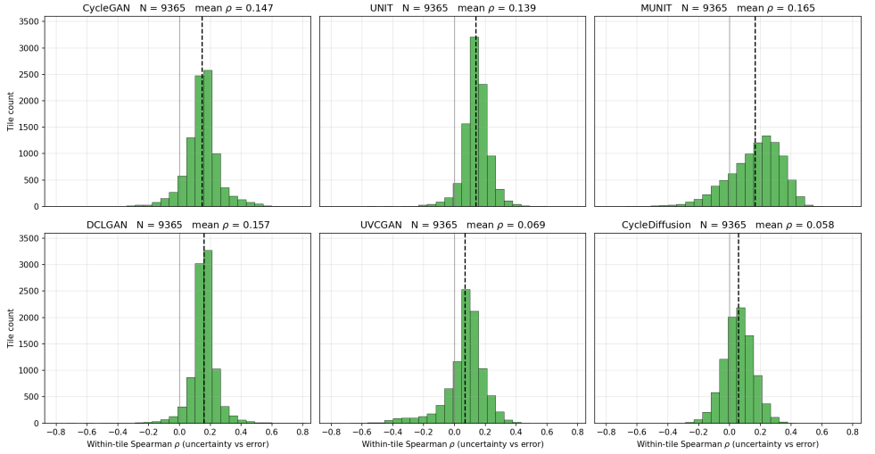
Figure S3: Distribution of within-tile Spearman r_s between pixel-level uncertainty U and cycle-reconstruction error E across the N=9,365 test tiles for each model family (top row: CycleGAN, UNIT, MUNIT; bottom row: DCLGAN, UVCAN, CycleDiffusion). The dashed vertical line marks the mean r_s . GAN-based families peak around r_s \approx 0.15 – 0.17 ; UVCAN and CycleDiffusion are centred near zero, confirming near-absent spatial calibration. The broad spread in all panels reflects high tile-to-tile variability.
