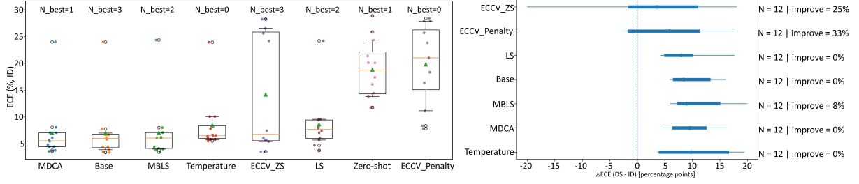
Figure 5: Left (ID): Boxplots of ECE (%) per method across backbones (IQR boxes, 10–90% whiskers, \blacktriangle mean, colored dots = backbone points, hollow circles = outliers). N_{\text{best}} shows the number of times it performs best across backbones. Lower, tighter boxes = more consistent ID calibration. Right (DS): Forest plot summarizing how each method’s ECE changes from ID to DS across backbones (dot = median, thick bar = IQR, thin line = 10–90%, dashed line at zero change), right text reports N backbones and improve % (share of backbones that get lower ECE in DS).
