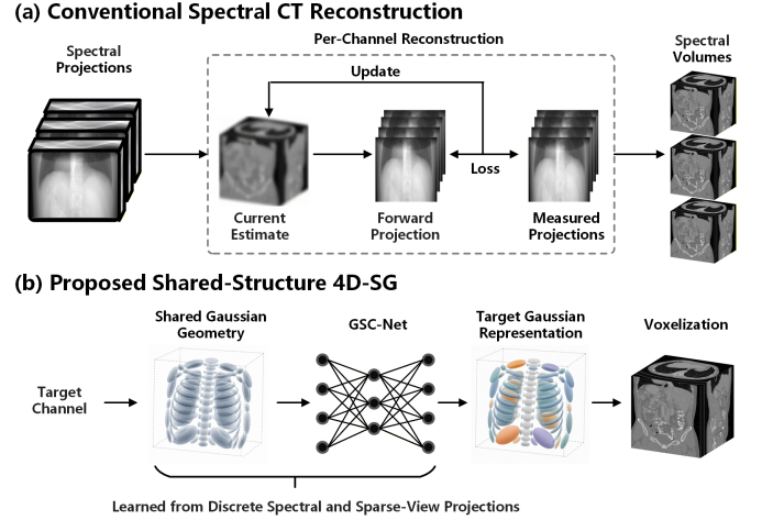
Fig. 1. Conceptual comparison. (a) Conventional methods reconstruct each spectral channel through an independent iterative process. (b) 4D-SG learns shared Gaussian geometry and GSC-Net from discrete spectral measurements and sparse-view projections and generates the Gaussian representation of a target channel for voxelization, supporting reconstruction and prediction of observed and unobserved spectral channels.
