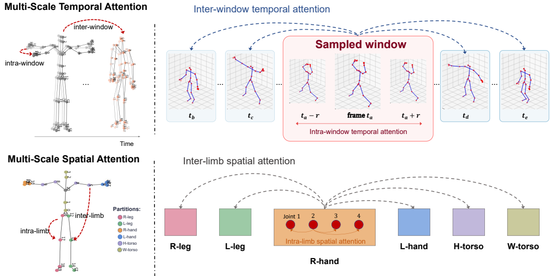
Figure 5: Multi-Scale Spatio-Temporal Attention Module. The temporal branch models short- and long-range motion dependencies through intra-window and inter-window attention, respectively, while the spatial branch captures local and global body interactions through intra-limb and inter-limb attention over predefined skeleton partitions.
