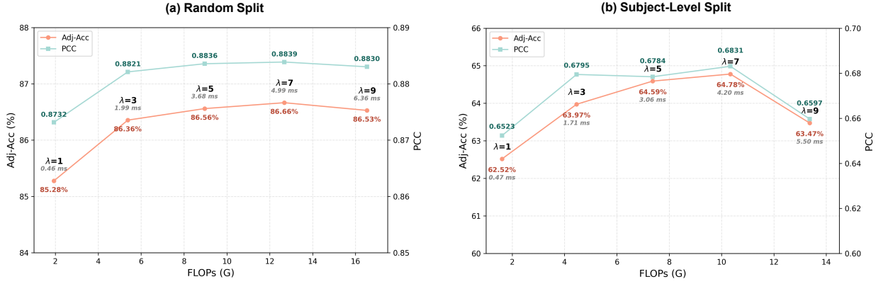
Figure 10: Sensitivity analysis of the number of candidate states \lambda in Pose2Muscle.
