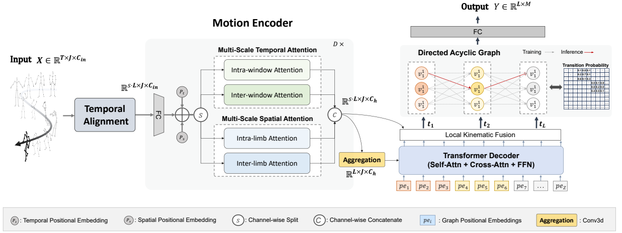
Figure 3: The framework of Pose2Muscle. We propose an MS-ST attention module in the motion encoder to learn motion features relevant to muscle activity estimation. The encoded features are fed into the muscle decoder, where a directed acyclic graph is constructed to mitigate uncertainty in muscle activity estimation.
