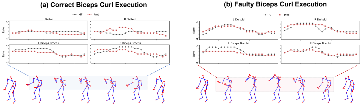
Figure 11: Prediction results for the biceps curl exercise. The masked regions highlight pose discrepancies, which may contribute to differences in muscle activation estimation.
