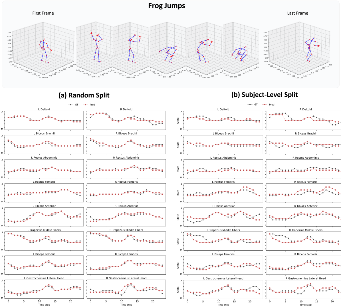
Figure 12: Qualitative results of Pose2Muscle on Frog Jumps. Each subplot visualizes sixteen muscles, where the horizontal axis corresponds to time steps and the vertical axis represents muscle activity types. ● and ● represent the ground truth and predicted labels, respectively.
