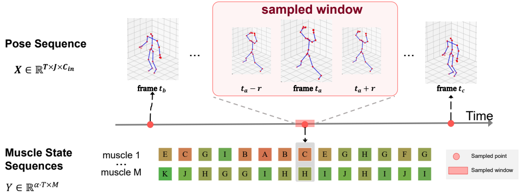
Figure 4: Temporal Sampling Alignment between Pose and Muscle. Point-to-window temporal alignment between muscle-state and pose sequences, where each discrete muscle-state sample is associated with a corresponding local pose window.
