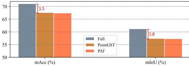
Fig. 5. Comparisons of mAcc and mIoU on the S3DIS dataset.
