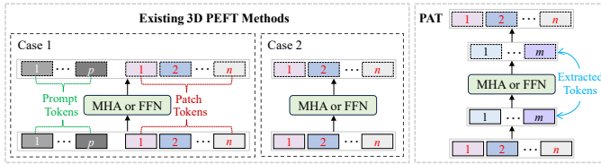
Fig. 1. Inference differences between PAT and existing 3D PEFT methods in MHA/FFN blocks. p , n , and m ( m < n ) represent the number of prompt tokens, patch tokens, and extracted tokens, respectively. Existing 3D PEFT methods include two cases: increasing the number of input tokens (Case 1) and keeping the input tokens unchanged (Case 2).
