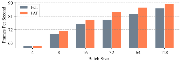
Fig. 9. Inference speed comparisons with varying batch sizes.
