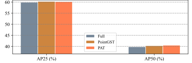
Fig. 7. Comparisons of AP25 and AP50 on the ScanNetV2 dataset.
