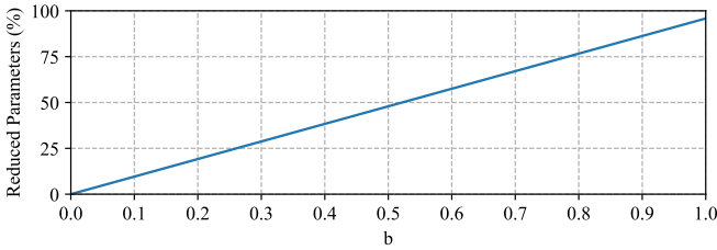
Fig. 3. Parameter reduction (%) achieved by BSLoRA compared to LoRA for varying values of b .
