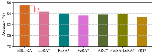
Fig. 4. Performance verification of BSLoRA.
