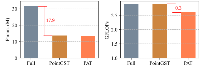
Fig. 8. Comparisons of the number of trainable parameters and the inference GFLOPs of the backbone on the ScanNetV2 dataset.
