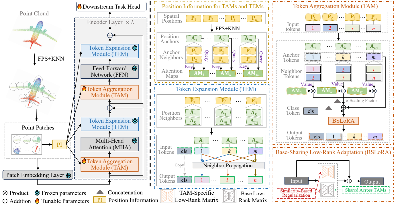
Fig. 2. Illustration of PAT. For the convenience of presentation, the 3D spatial information required by TAMs and TEMs, including point patch positions \{\mathbf{P}_i\}_{i=1}^n , position anchors \{\mathbf{A}_i\}_{i=1}^m , and the attention maps \{\mathbf{AM}_i\}_{i=1}^m between position anchors and their neighbors, is processed within the PI module. TAMs, inserted before MHA or FFN blocks, extract m anchor tokens from n patch tokens based on the provided information, and then apply BSLoRA to effectively adapt these anchor tokens to downstream tasks in a parameter-efficient way.
