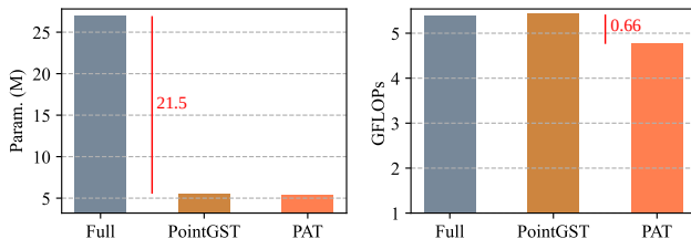
Fig. 6. Comparisons of the number of trainable parameters and the inference GFLOPs of the backbone on the S3DIS dataset.
