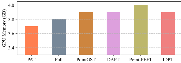
Fig. 10. Comparisons of GPU memory at a batch size of 8.
