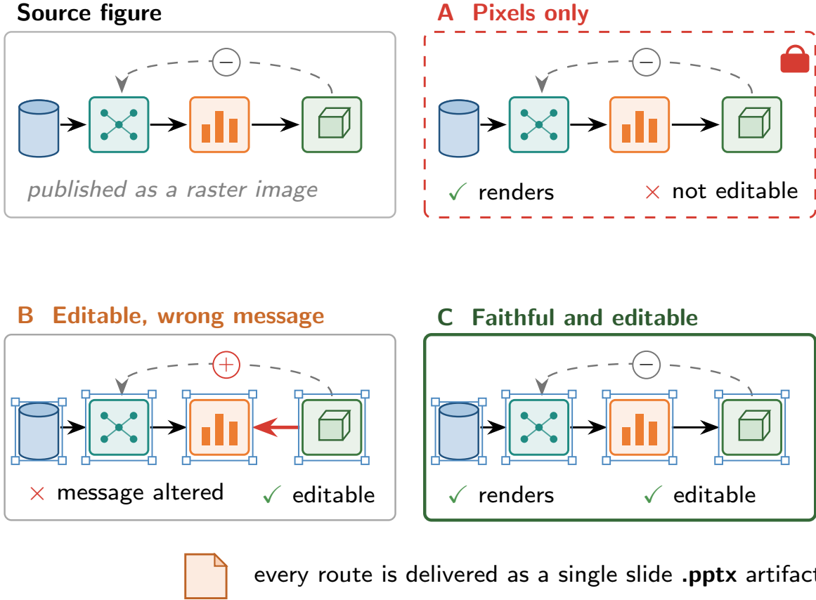
Figure 1: The reconstruction contract. Top left: a source overview figure, published as a raster image. A, B, and C: three candidate reconstructions, a raster paste (A), an editable slide with a reversed arrow and an altered sign (B), and a faithful editable slide (C). Badges mark whether each route renders like the source and remains natively editable. Every route delivers a PPTX artifact with a single slide.
