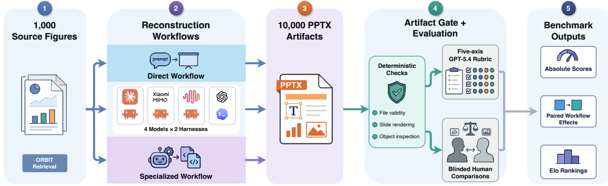
Figure 3: The ReFigBench pipeline. From left to right, ORBIT retrieves 1,000 source figures. Four models reconstruct each figure under two workflows, with GPT-5.5 additionally running inside both commercial harnesses, yielding ten configurations. The resulting 10,000 PPTX artifacts pass deterministic artifact checks. A rubric with five axes and blinded pairwise human comparisons score them. The outputs are absolute scores, paired workflow effects, and human Elo rankings.
