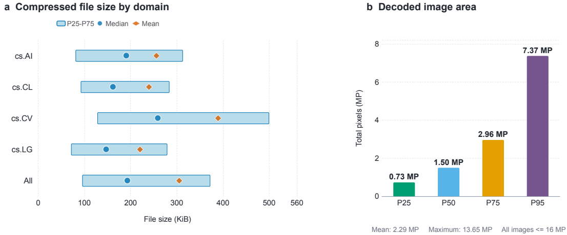
Figure 7: Input-image size profile. (a) Interquartile file-size range by source domain with median and mean markers. (b) Percentiles of decoded pixel area. Compressed file size understates the memory and rendering burden of high-resolution scientific figures.
