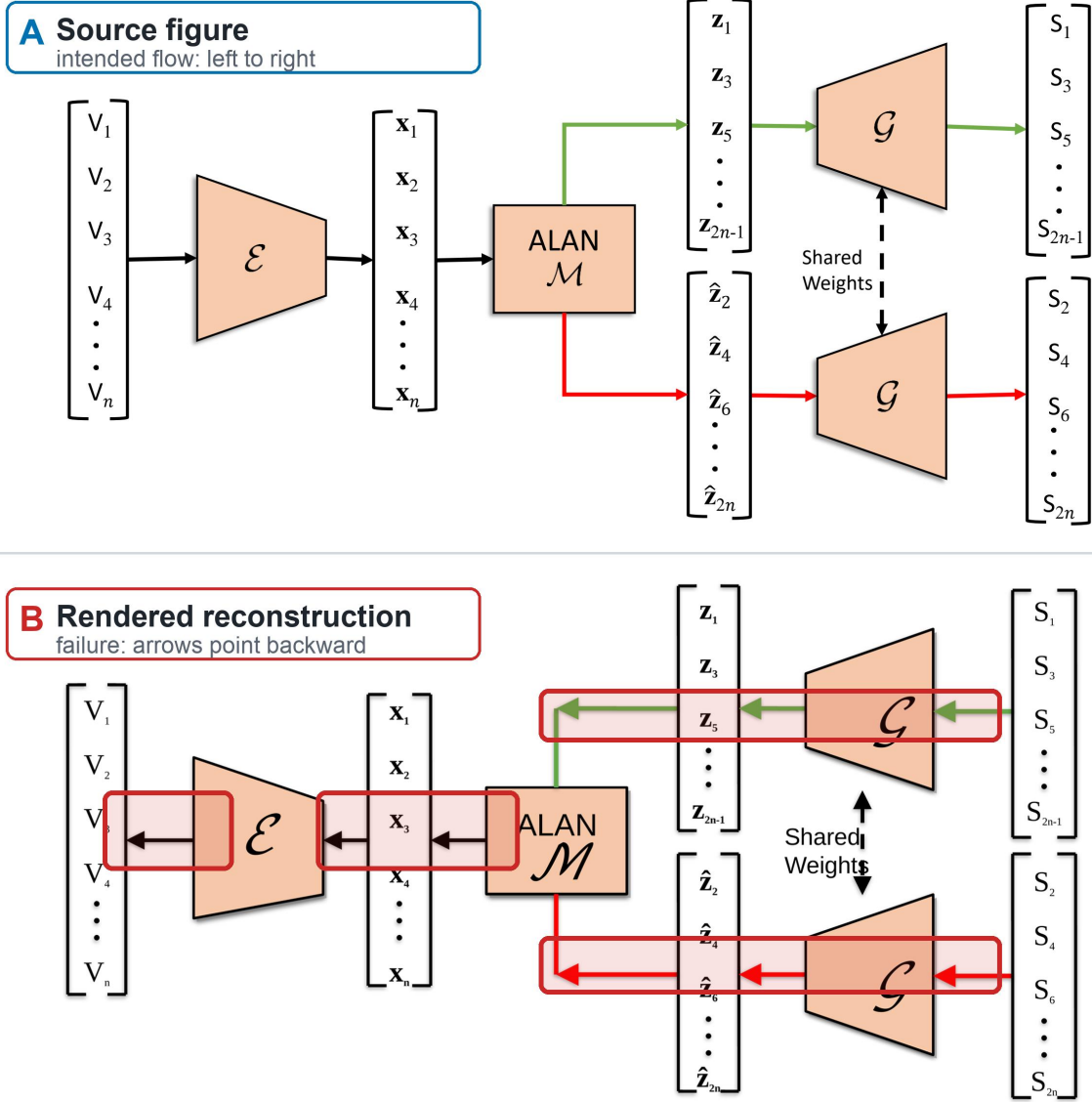
Figure 6: Annotated case study pair. The top panel is the source benchmark figure, a video restoration pipeline that reads left to right through an encoder, a central attention module, and two weight sharing decoders. The bottom panel is the rendered reconstruction, which reproduces the blocks, frame stacks, colored branches, and dashed weight sharing tie while reversing the arrows highlighted in red.
