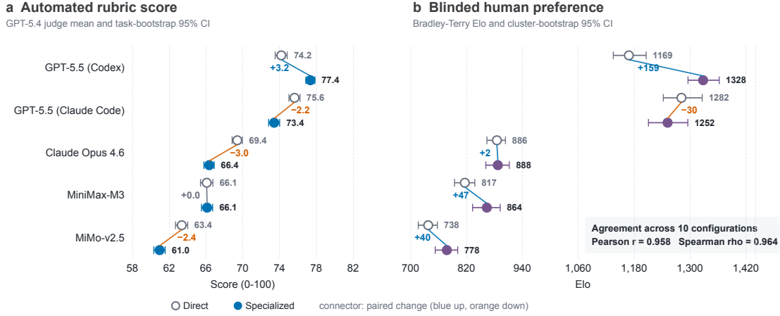
Figure 5: Rubric scores (left) and human Bradley-Terry Elo (right). Each row pairs the direct (hollow) and specialized (filled) configurations of one model and harness. The connector shows the paired change, and error bars are 95% confidence intervals.
