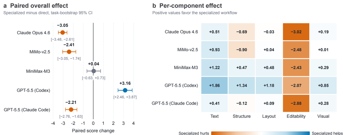
Figure 4: Paired specialized minus direct effects. Left: overall score change per model and harness pair, with the estimate and 95% bootstrap interval beside each marker. Right: changes by component. Positive values favor the specialized workflow.
