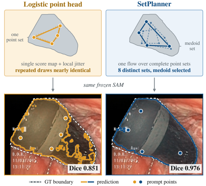
Fig. 1. Point-source contrast. Left: a single score map with local jitter. Right: one flow over complete point sets. Each polygon links one K=4 point set. The qualitative pair uses an official Kvasir-Instrument test frame.
