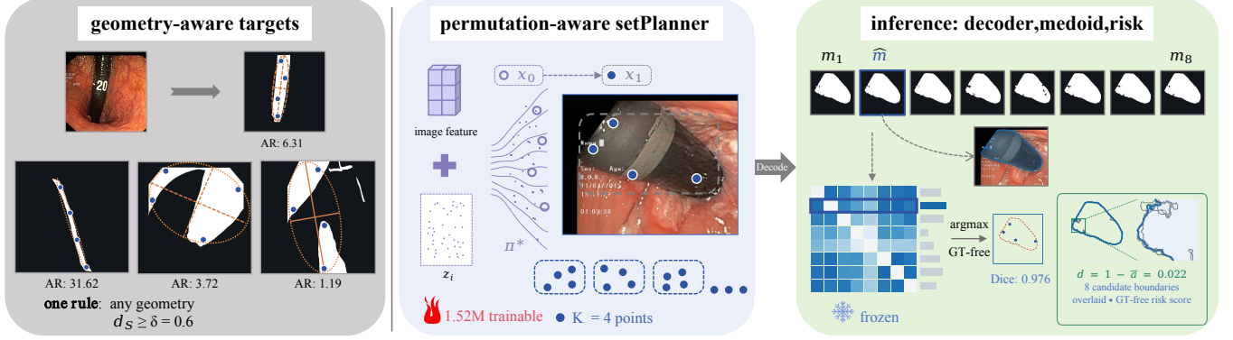
Fig. 2. SetPlanner, left to right. Targets x_1 come from the eroded foreground under a Mahalanobis floor in the foreground’s second-moment frame; AR = axis ratio. In model coordinates [-1, 1] , the optimal assignment \pi^* pairs a Gaussian draw with the target set. M=8 decoded candidates reduce to one by a consensus readout; disagreement d ranks failures without GT.
